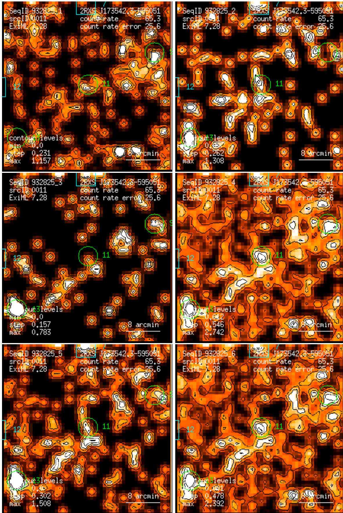
Figure 11: RASS 932825: detection 0011: band rate images, Gaussian filter: (1) PSPC channels 11 – 41, (2) 52 – 90, (3) 91 – 201, (4) 11 – 235, (5) 52 – 201, (6) 11 – 201. Broad band rates in counts/ks. Band rate contour levels in counts/ks/arcmin 2 .
