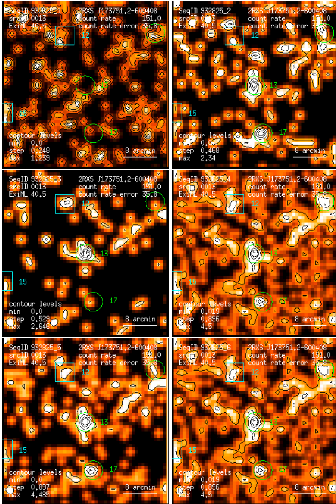
Figure 13: RASS 932825: detection 0013: band rate images, Gaussian filter: (1) PSPC channels 11 – 41, (2) 52 – 90, (3) 91 – 201, (4) 11 – 235, (5) 52 – 201, (6) 11 – 201. Broad band rates in counts/ks. Band rate contour levels in counts/ks/arcmin 2 .
