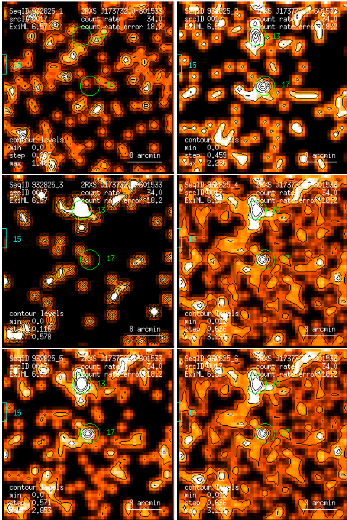
Figure 17: RASS 932825: detection 0017: band rate images, Gaussian filter: (1) PSPC channels 11 – 41, (2) 52 – 90, (3) 91 – 201, (4) 11 – 235, (5) 52 – 201, (6) 11 – 201. Broad band rates in counts/ks. Band rate contour levels in counts/ks/arcmin 2 .
