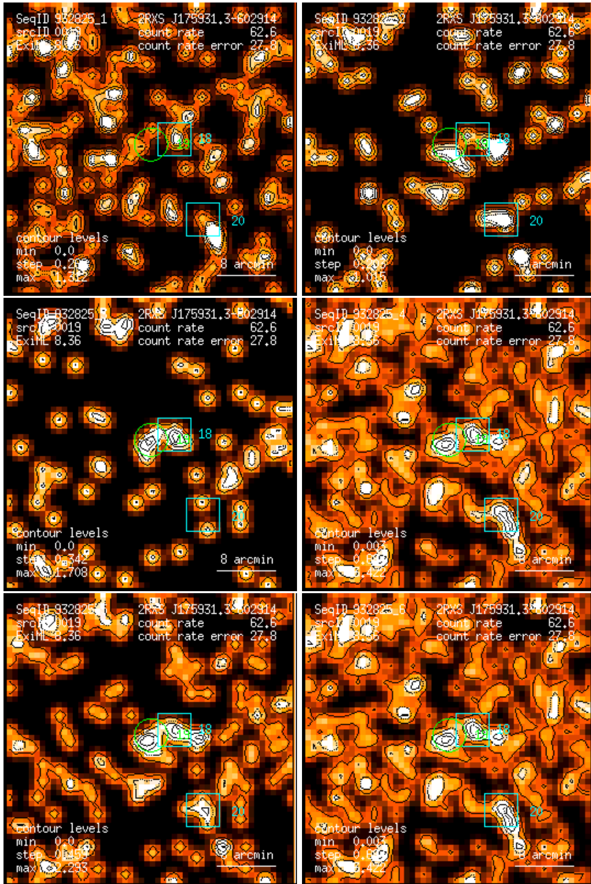
Figure 19: RASS 932825: detection 0019: band rate images, Gaussian filter: (1) PSPC channels 11 – 41, (2) 52 – 90, (3) 91 – 201, (4) 11 – 235, (5) 52 – 201, (6) 11 – 201. Broad band rates in counts/ks. Band rate contour levels in counts/ks/arcmin 2 .
