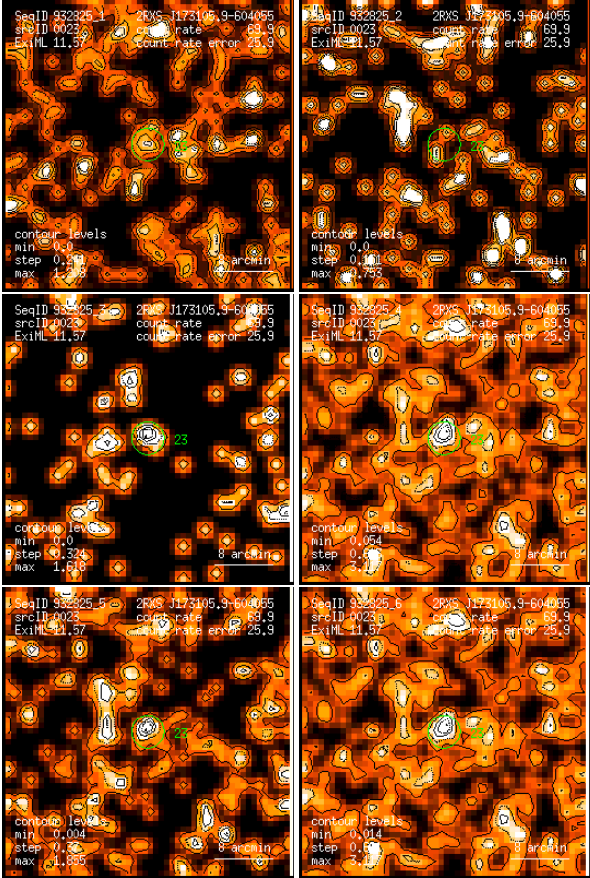
Figure 23: RASS 932825: detection 0023: band rate images, Gaussian filter: (1) PSPC channels 11 – 41, (2) 52 – 90, (3) 91 – 201, (4) 11 – 235, (5) 52 – 201, (6) 11 – 201. Broad band rates in counts/ks. Band rate contour levels in counts/ks/arcmin 2 .
