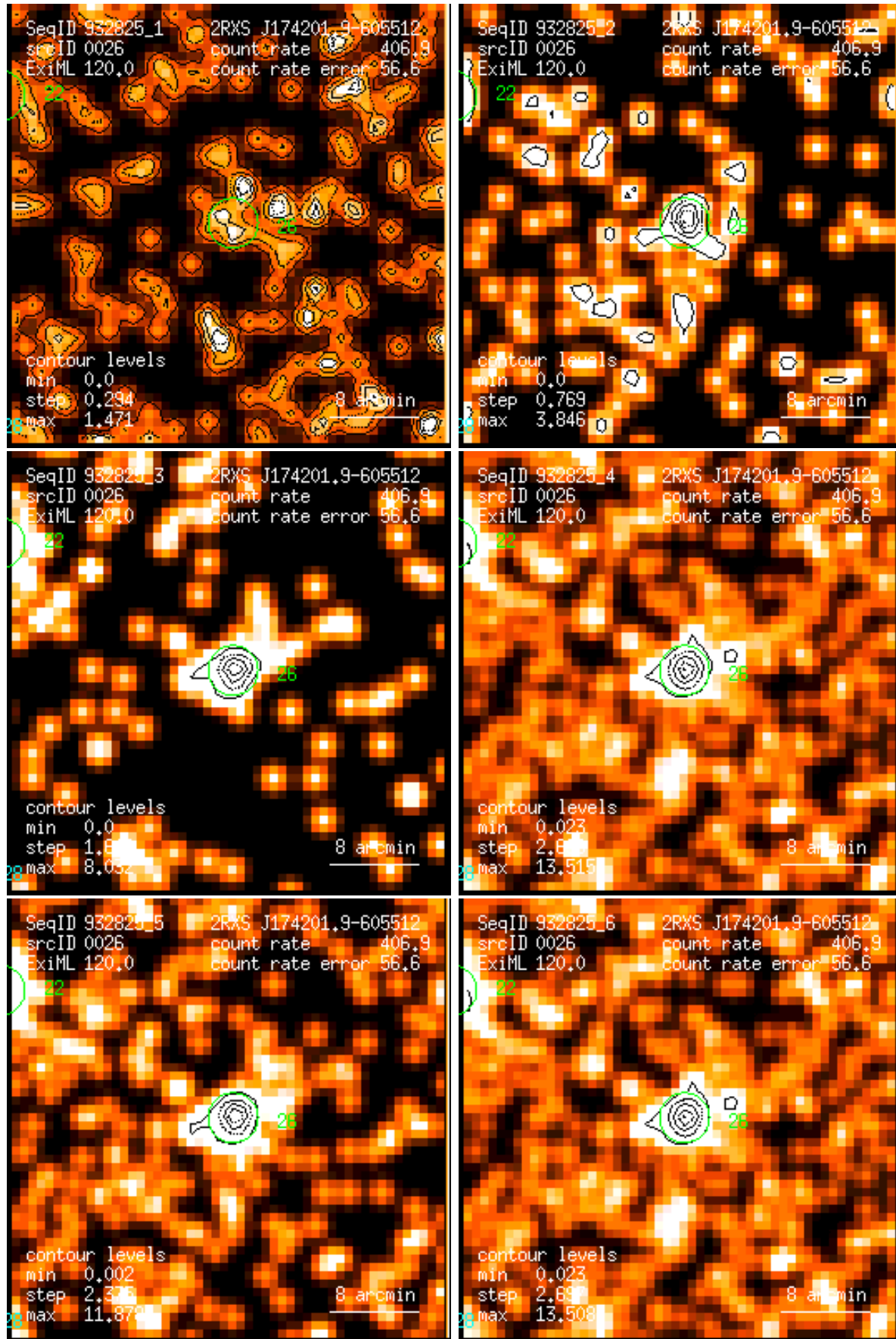
Figure 26: RASS 932825: detection 0026: band rate images, Gaussian filter: (1) PSPC channels 11 – 41, (2) 52 – 90, (3) 91 – 201, (4) 11 – 235, (5) 52 – 201, (6) 11 – 201. Broad band rates in counts/ks. Band rate contour levels in counts/ks/arcmin 2 .
