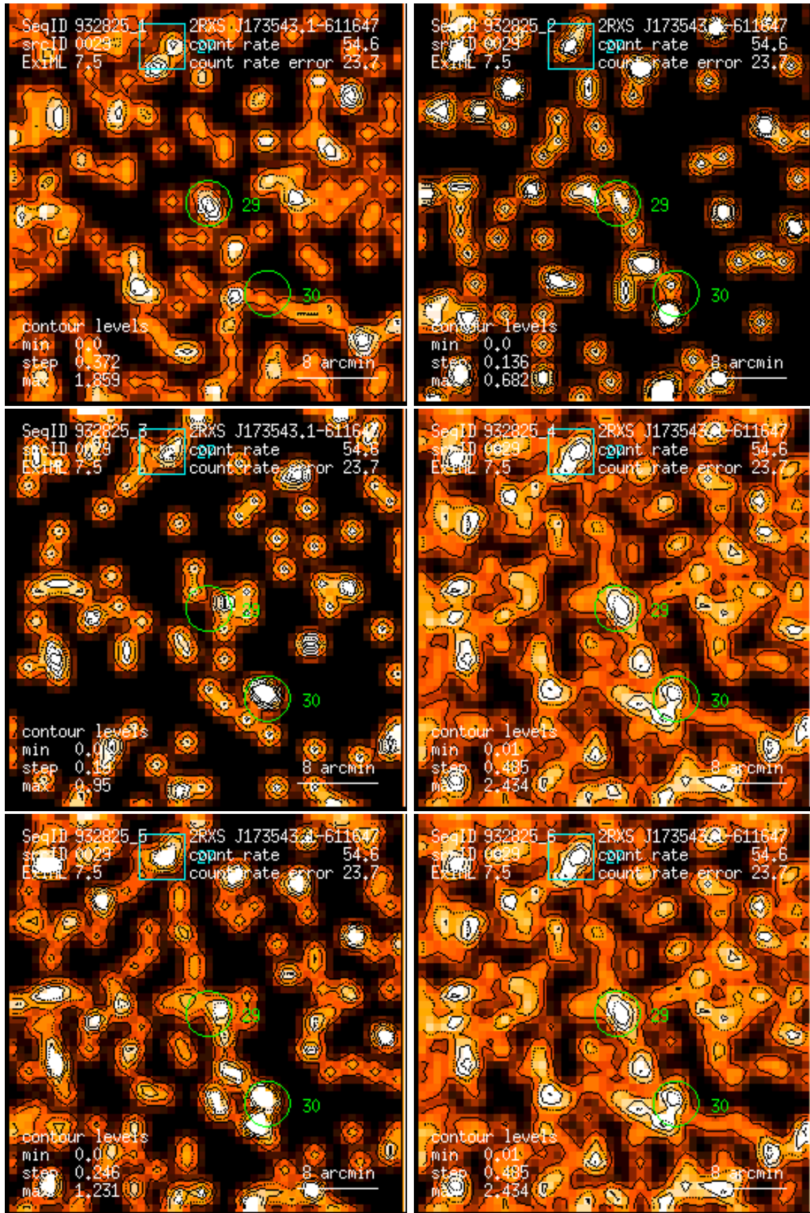
Figure 29: RASS 932825: detection 0029: band rate images, Gaussian filter: (1) PSPC channels 11 – 41, (2) 52 – 90, (3) 91 – 201, (4) 11 – 235, (5) 52 – 201, (6) 11 – 201. Broad band rates in counts/ks. Band rate contour levels in counts/ks/arcmin 2 .
