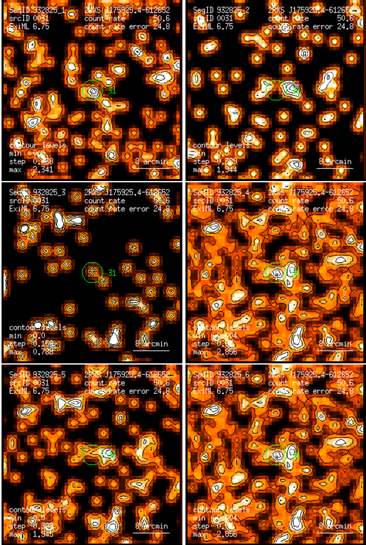
Figure 31: RASS 932825: detection 0031: band rate images, Gaussian filter: (1) PSPC channels 11 – 41, (2) 52 – 90, (3) 91 – 201, (4) 11 – 235, (5) 52 – 201, (6) 11 – 201. Broad band rates in counts/ks. Band rate contour levels in counts/ks/arcmin 2 .
