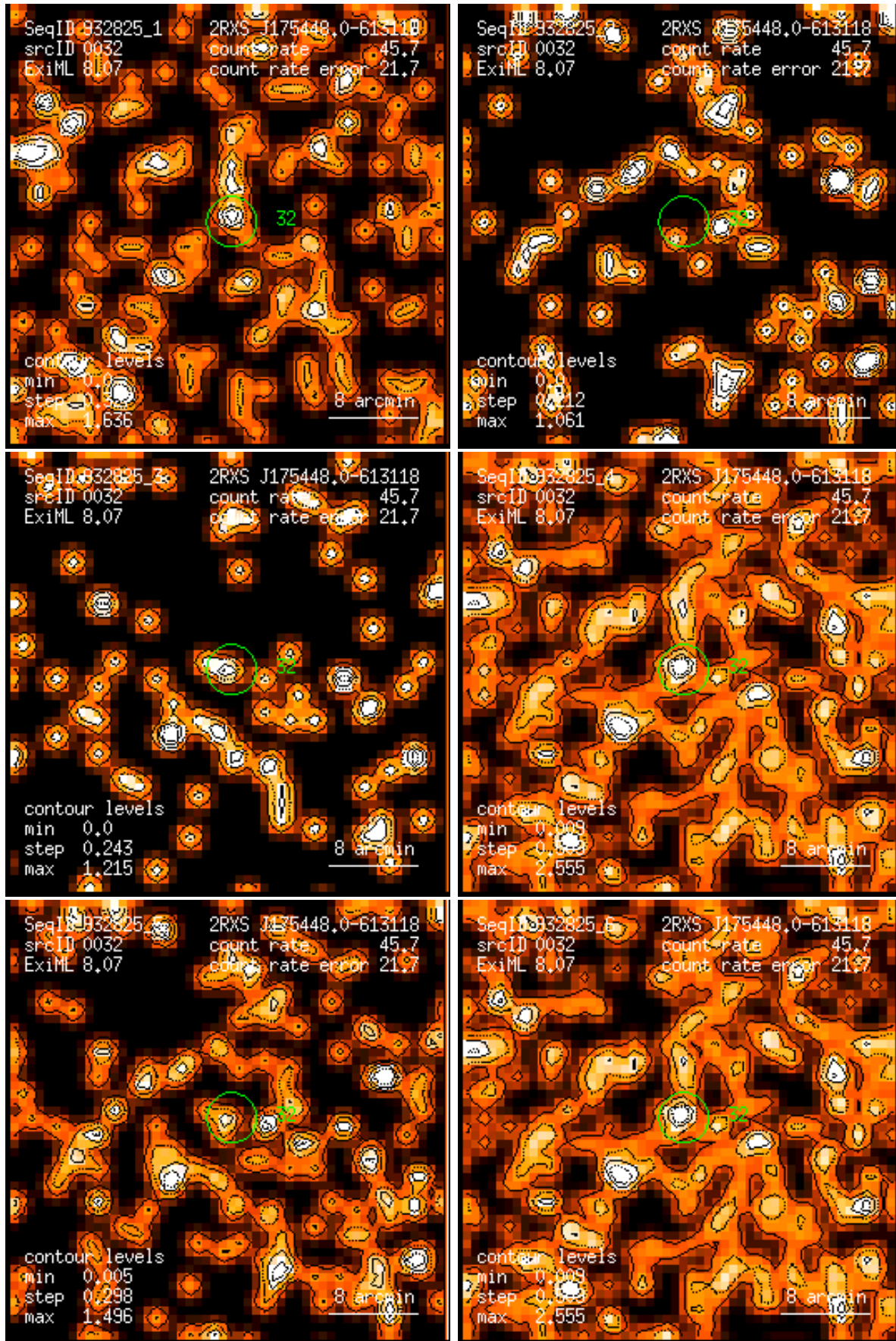
Figure 32: RASS 932825: detection 0032: band rate images, Gaussian filter: (1) PSPC channels 11 – 41, (2) 52 – 90, (3) 91 – 201, (4) 11 – 235, (5) 52 – 201, (6) 11 – 201. Broad band rates in counts/ks. Band rate contour levels in counts/ks/arcmin 2 .
