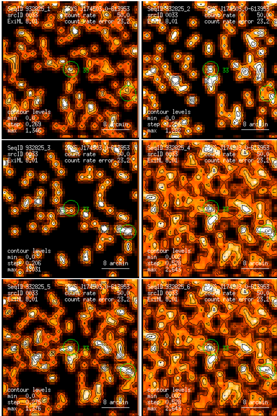
Figure 33: RASS 932825: detection 0033: band rate images, Gaussian filter: (1) PSPC channels 11 – 41, (2) 52 – 90, (3) 91 – 201, (4) 11 – 235, (5) 52 – 201, (6) 11 – 201. Broad band rates in counts/ks. Band rate contour levels in counts/ks/arcmin 2 .
