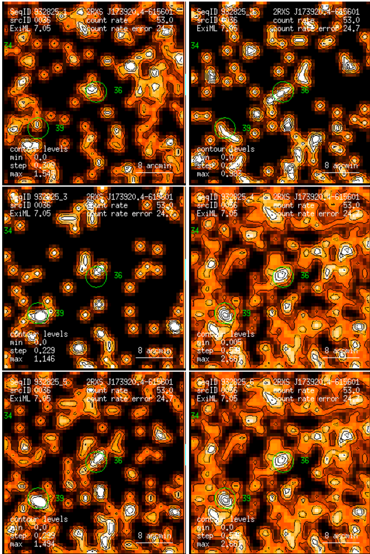
Figure 36: RASS 932825: detection 0036: band rate images, Gaussian filter: (1) PSPC channels 11 – 41, (2) 52 – 90, (3) 91 – 201, (4) 11 – 235, (5) 52 – 201, (6) 11 – 201. Broad band rates in counts/ks. Band rate contour levels in counts/ks/arcmin 2 .
