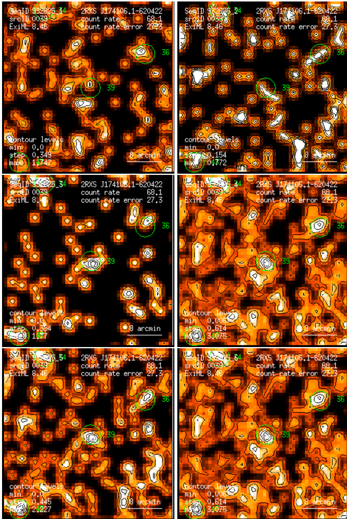
Figure 39: RASS 932825: detection 0039: band rate images, Gaussian filter: (1) PSPC channels 11 – 41, (2) 52 – 90, (3) 91 – 201, (4) 11 – 235, (5) 52 – 201, (6) 11 – 201. Broad band rates in counts/ks. Band rate contour levels in counts/ks/arcmin 2 .
