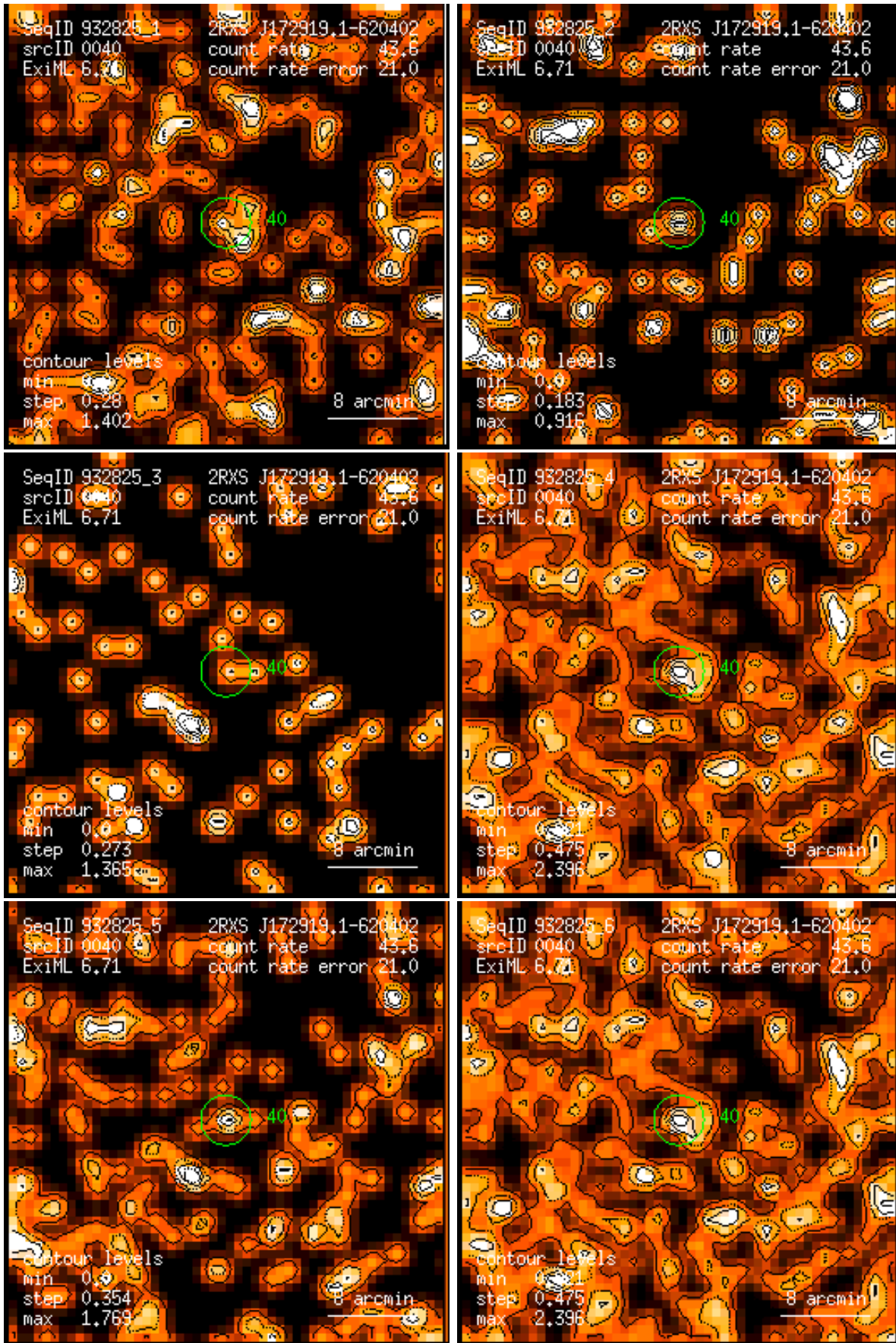
Figure 40: RASS 932825: detection 0040: band rate images, Gaussian filter: (1) PSPC channels 11 – 41, (2) 52 – 90, (3) 91 – 201, (4) 11 – 235, (5) 52 – 201, (6) 11 – 201. Broad band rates in counts/ks. Band rate contour levels in counts/ks/arcmin 2 .
