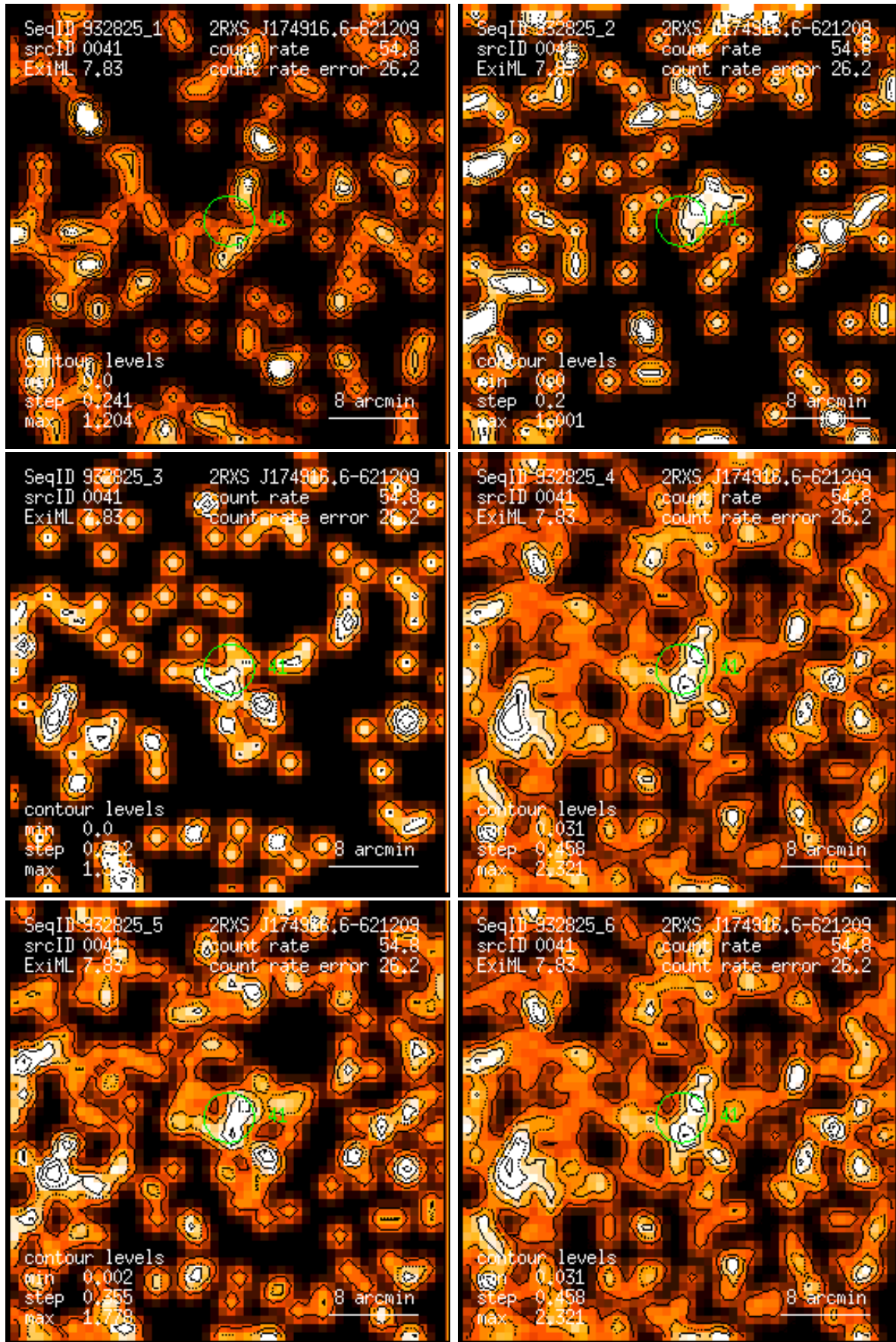
Figure 41: RASS 932825: detection 0041: band rate images, Gaussian filter: (1) PSPC channels 11 – 41, (2) 52 – 90, (3) 91 – 201, (4) 11 – 235, (5) 52 – 201, (6) 11 – 201. Broad band rates in counts/ks. Band rate contour levels in counts/ks/arcmin 2 .
