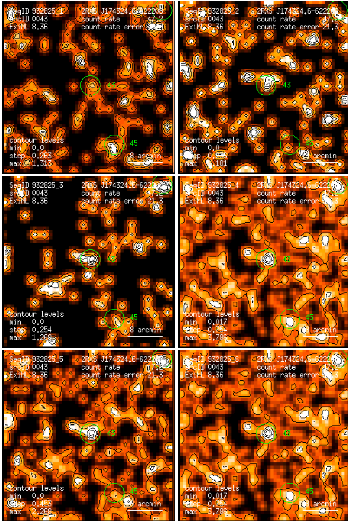
Figure 43: RASS 932825: detection 0043: band rate images, Gaussian filter: (1) PSPC channels 11 – 41, (2) 52 – 90, (3) 91 – 201, (4) 11 – 235, (5) 52 – 201, (6) 11 – 201. Broad band rates in counts/ks. Band rate contour levels in counts/ks/arcmin 2 .
