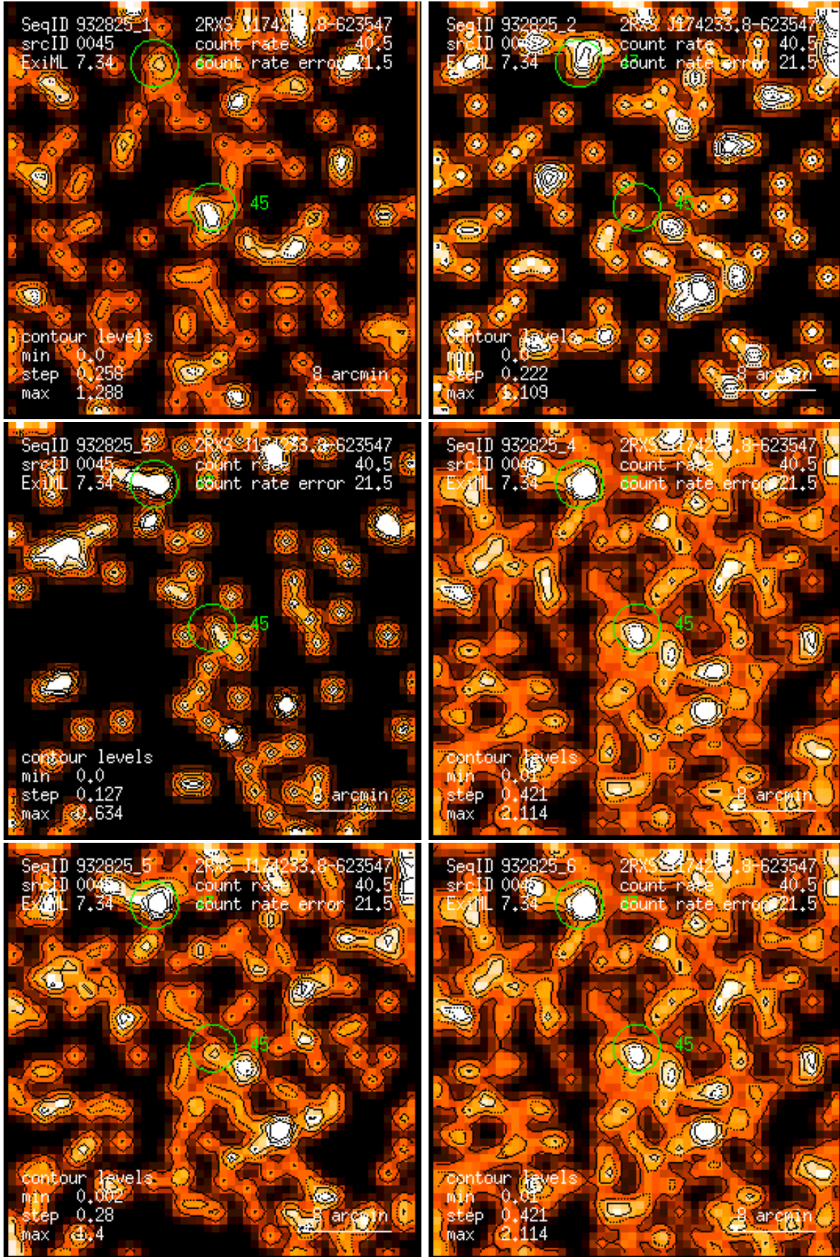
Figure 45: RASS 932825: detection 0045: band rate images, Gaussian filter: (1) PSPC channels 11 – 41, (2) 52 – 90, (3) 91 – 201, (4) 11 – 235, (5) 52 – 201, (6) 11 – 201. Broad band rates in counts/ks. Band rate contour levels in counts/ks/arcmin 2 .
