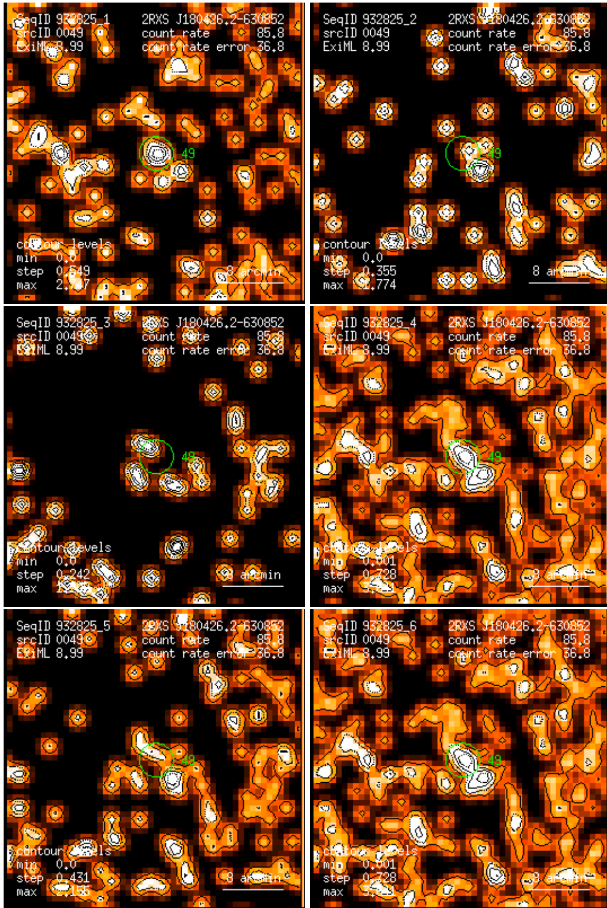
Figure 49: RASS 932825: detection 0049: band rate images, Gaussian filter: (1) PSPC channels 11 – 41, (2) 52 – 90, (3) 91 – 201, (4) 11 – 235, (5) 52 – 201, (6) 11 – 201. Broad band rates in counts/ks. Band rate contour levels in counts/ks/arcmin 2 .
