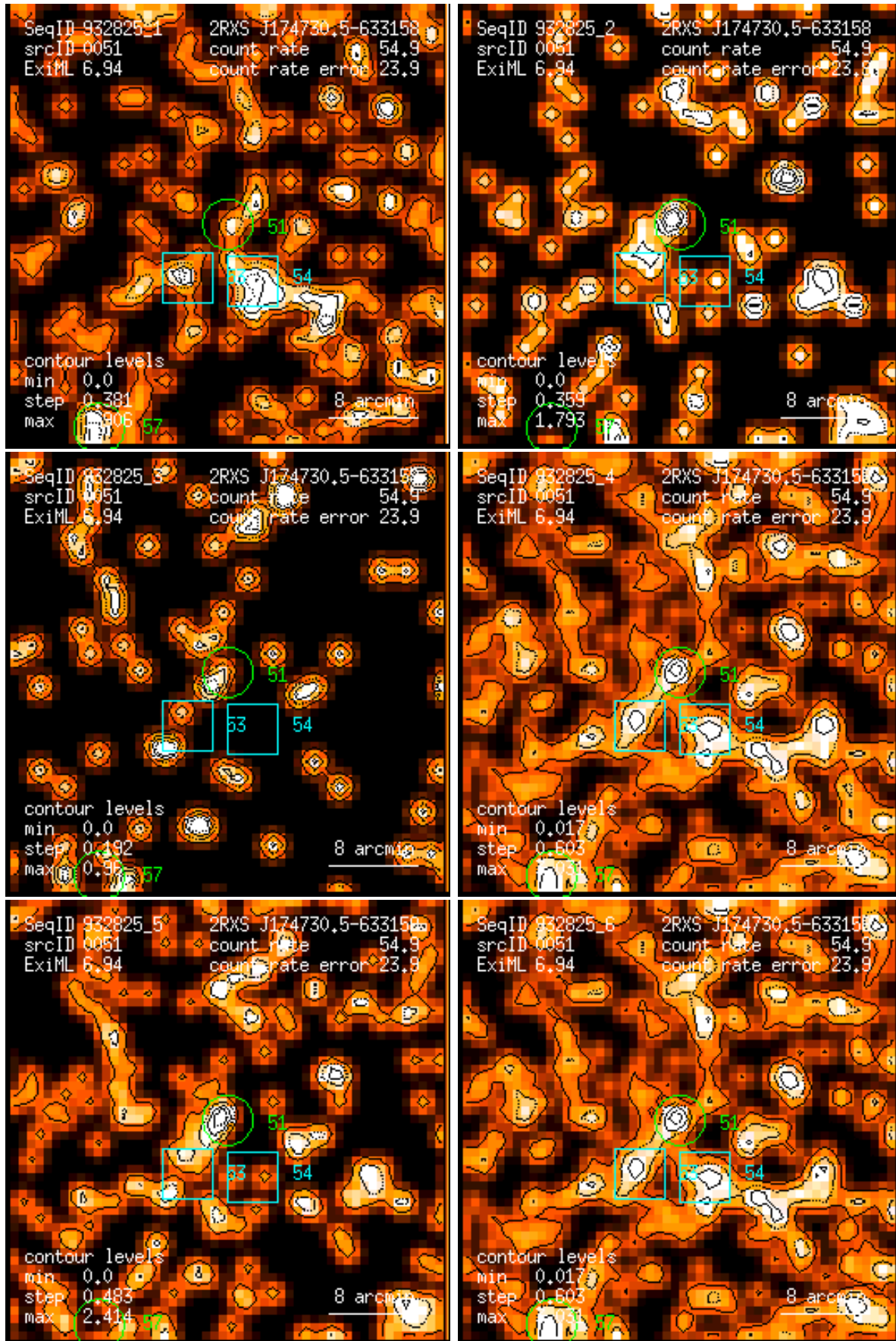
Figure 51: RASS 932825: detection 0051: band rate images, Gaussian filter: (1) PSPC channels 11 – 41, (2) 52 – 90, (3) 91 – 201, (4) 11 – 235, (5) 52 – 201, (6) 11 – 201. Broad band rates in counts/ks. Band rate contour levels in counts/ks/arcmin 2 .
