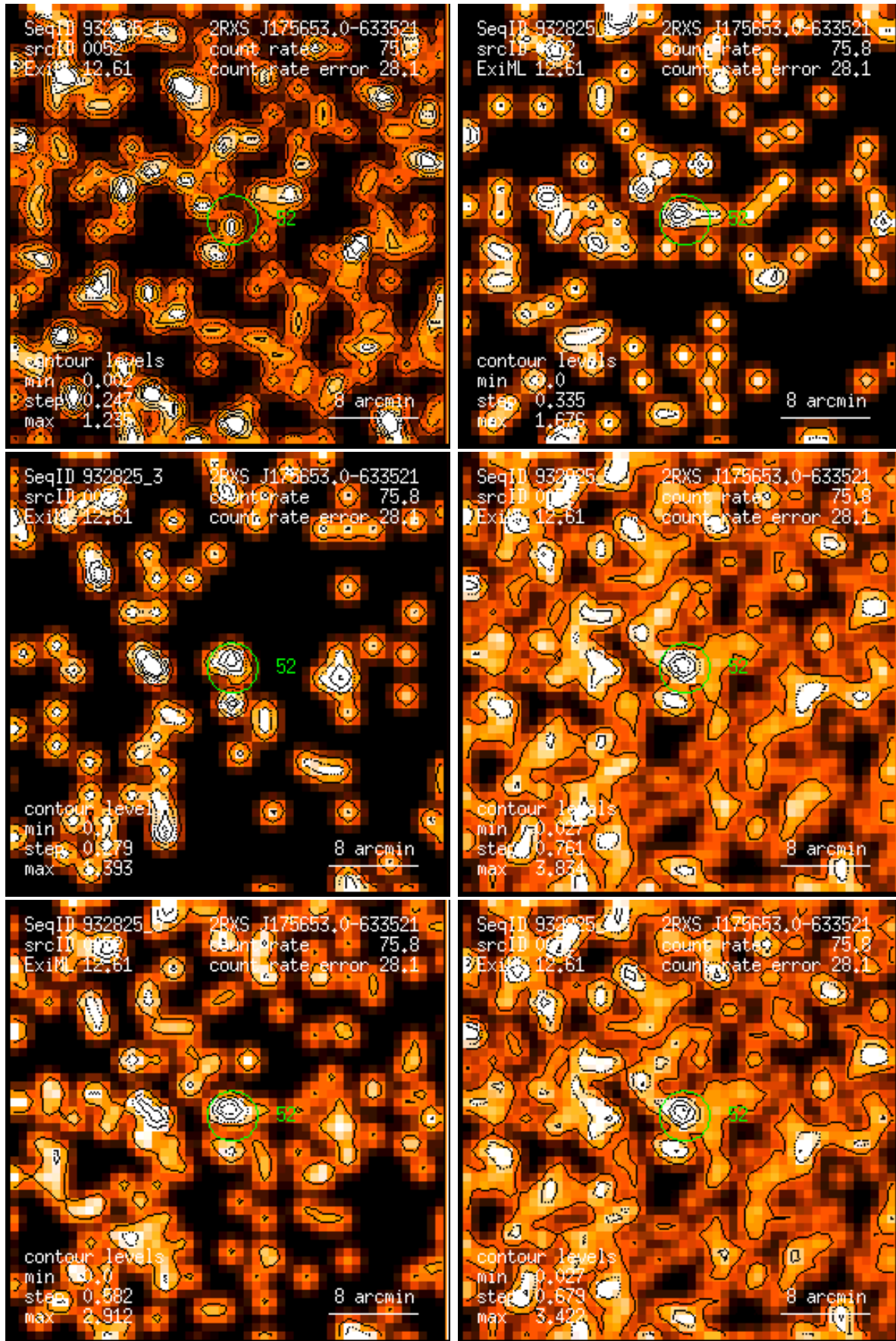
Figure 52: RASS 932825: detection 0052: band rate images, Gaussian filter: (1) PSPC channels 11 – 41, (2) 52 – 90, (3) 91 – 201, (4) 11 – 235, (5) 52 – 201, (6) 11 – 201. Broad band rates in counts/ks. Band rate contour levels in counts/ks/arcmin 2 .
