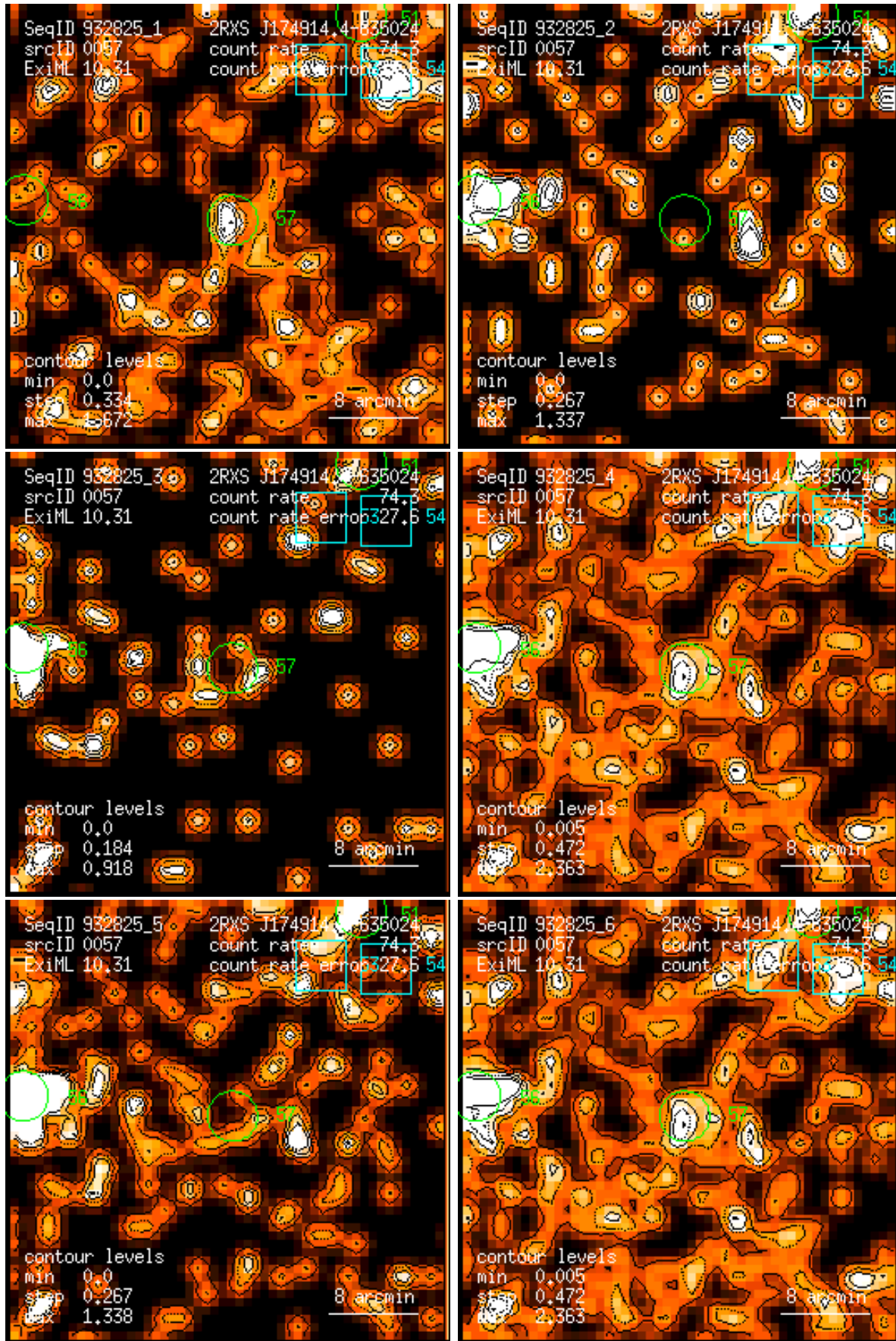
Figure 57: RASS 932825: detection 0057: band rate images, Gaussian filter: (1) PSPC channels 11 – 41, (2) 52 – 90, (3) 91 – 201, (4) 11 – 235, (5) 52 – 201, (6) 11 – 201. Broad band rates in counts/ks. Band rate contour levels in counts/ks/arcmin 2 .
