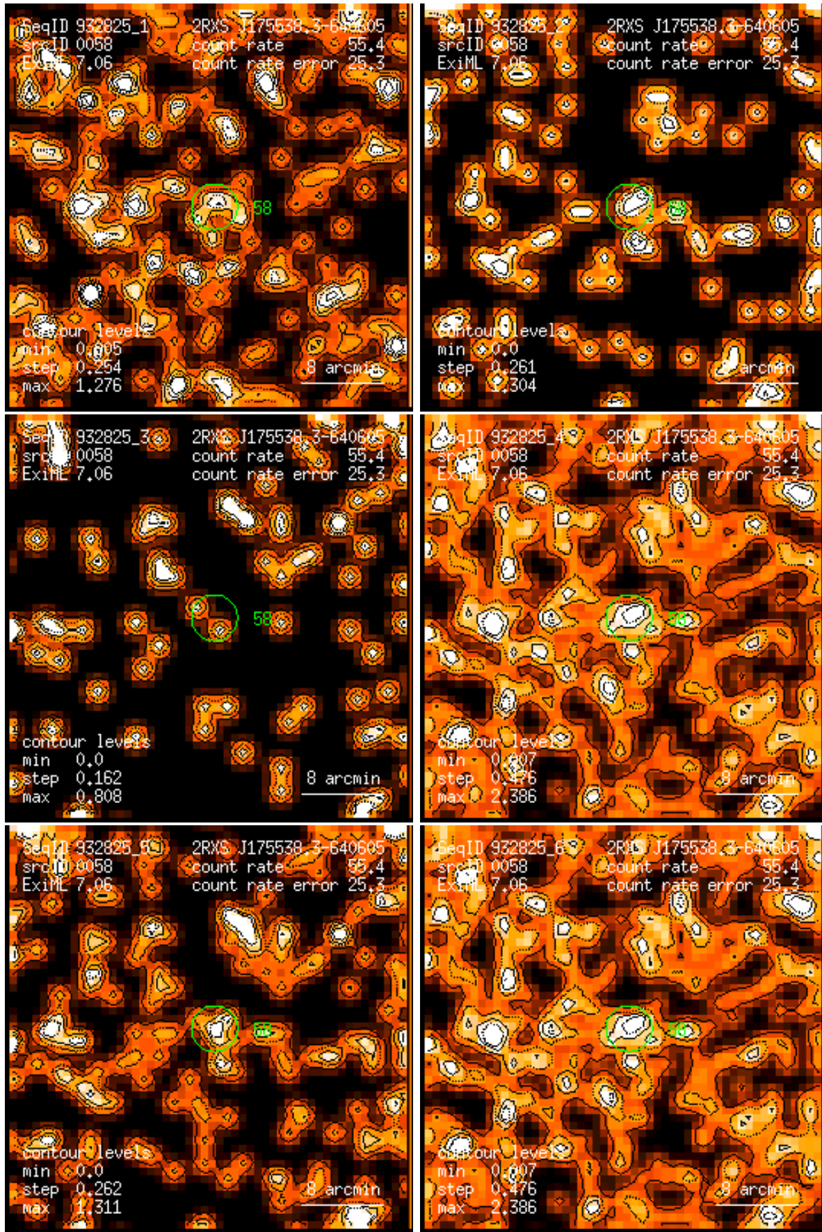
Figure 58: RASS 932825: detection 0058: band rate images, Gaussian filter: (1) PSPC channels 11 – 41, (2) 52 – 90, (3) 91 – 201, (4) 11 – 235, (5) 52 – 201, (6) 11 – 201. Broad band rates in counts/ks. Band rate contour levels in counts/ks/arcmin 2 .
