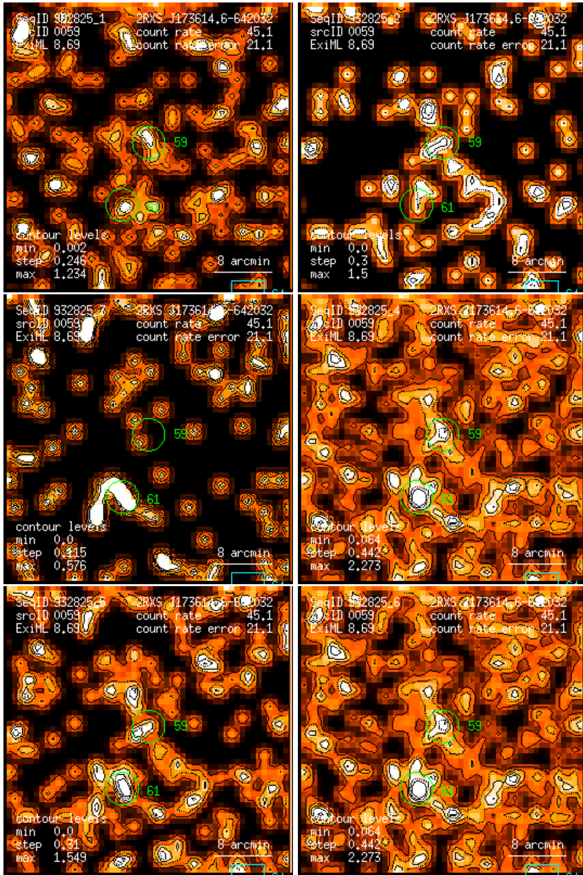
Figure 59: RASS 932825: detection 0059: band rate images, Gaussian filter: (1) PSPC channels 11 – 41, (2) 52 – 90, (3) 91 – 201, (4) 11 – 235, (5) 52 – 201, (6) 11 – 201. Broad band rates in counts/ks. Band rate contour levels in counts/ks/arcmin 2 .
