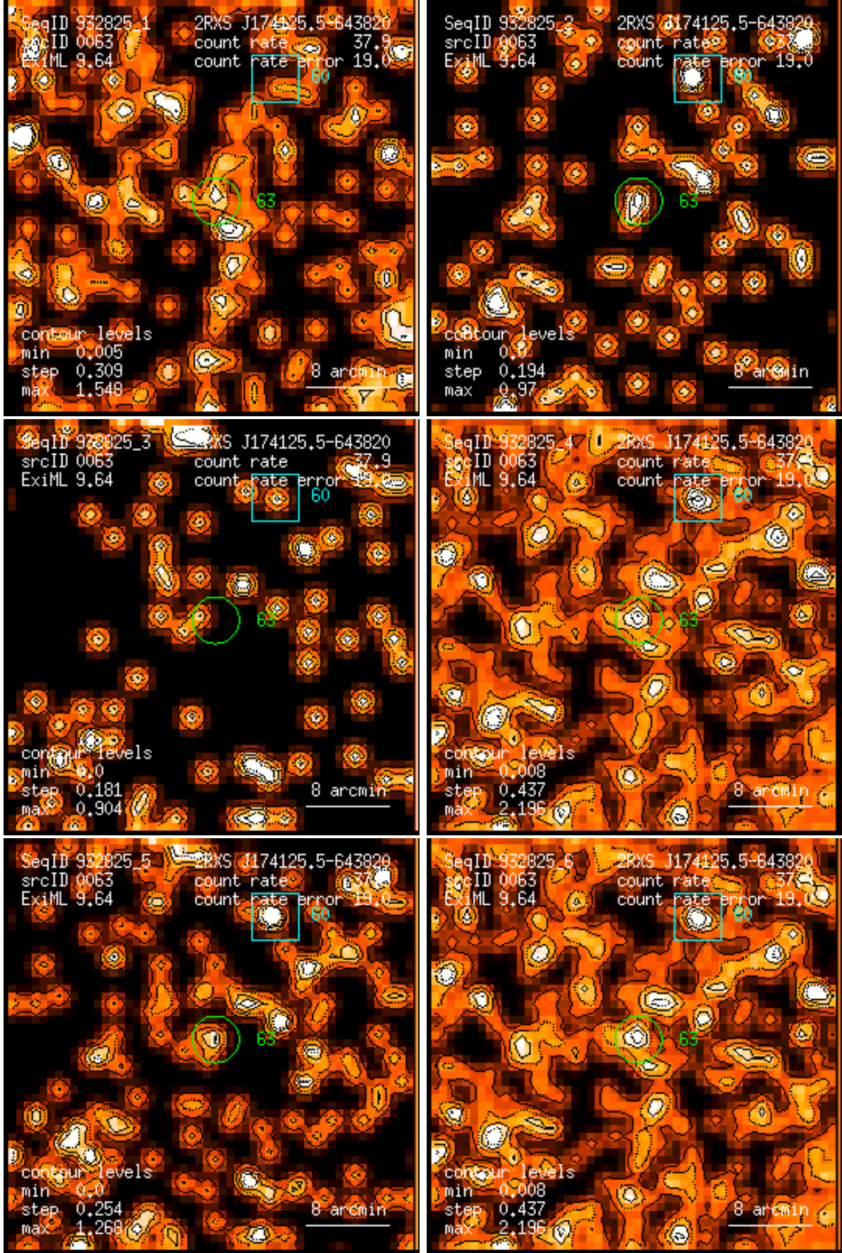
Figure 63: RASS 932825: detection 0063: band rate images, Gaussian filter: (1) PSPC channels 11 – 41, (2) 52 – 90, (3) 91 – 201, (4) 11 – 235, (5) 52 – 201, (6) 11 – 201. Broad band rates in counts/ks. Band rate contour levels in counts/ks/arcmin 2 .
