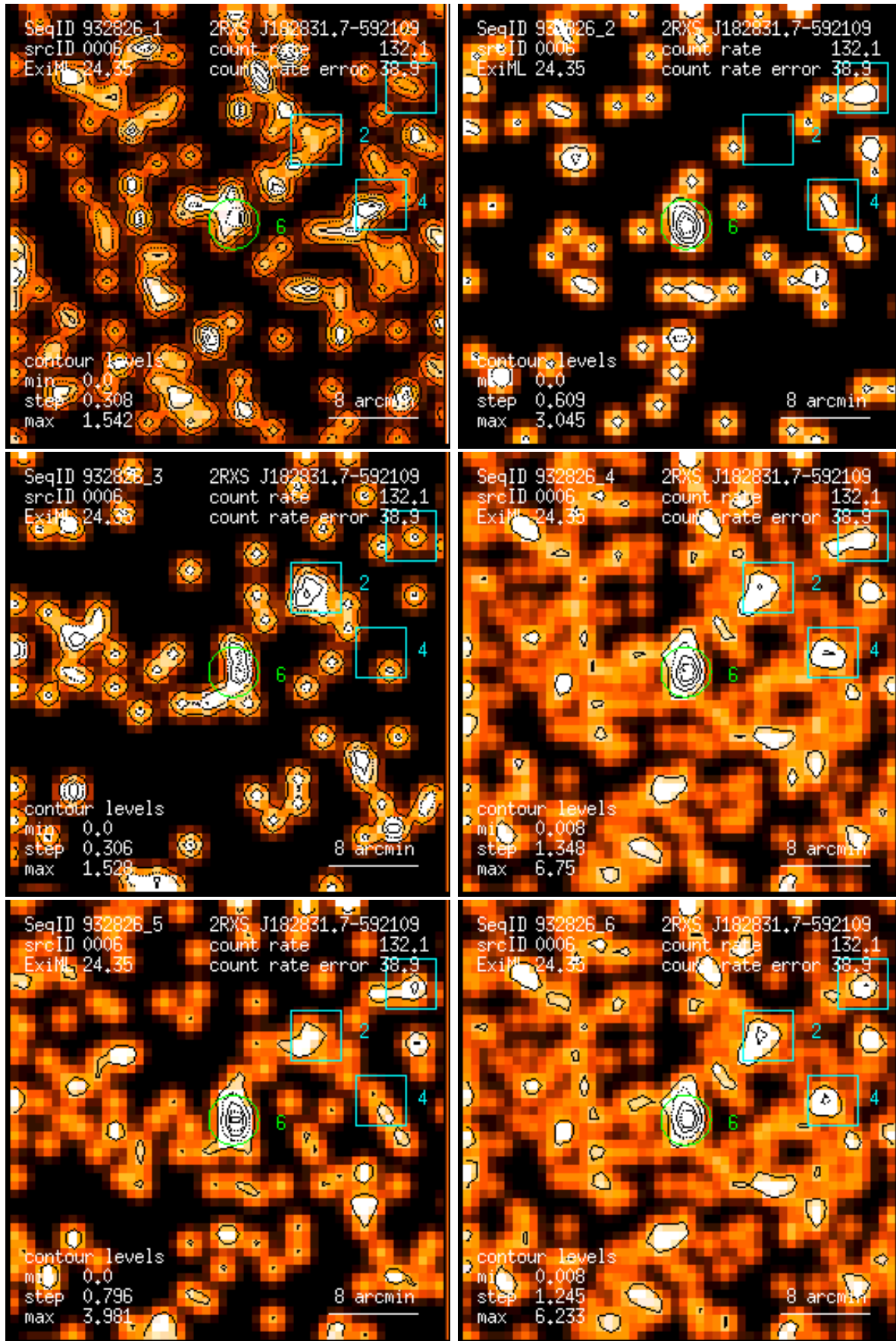
Figure 6: RASS 932826: detection 0006: band rate images, Gaussian filter: (1) PSPC channels 11 – 41, (2) 52 – 90, (3) 91 – 201, (4) 11 – 235, (5) 52 – 201, (6) 11 – 201. Broad band rates in counts/ks. Band rate contour levels in counts/ks/arcmin 2 .
