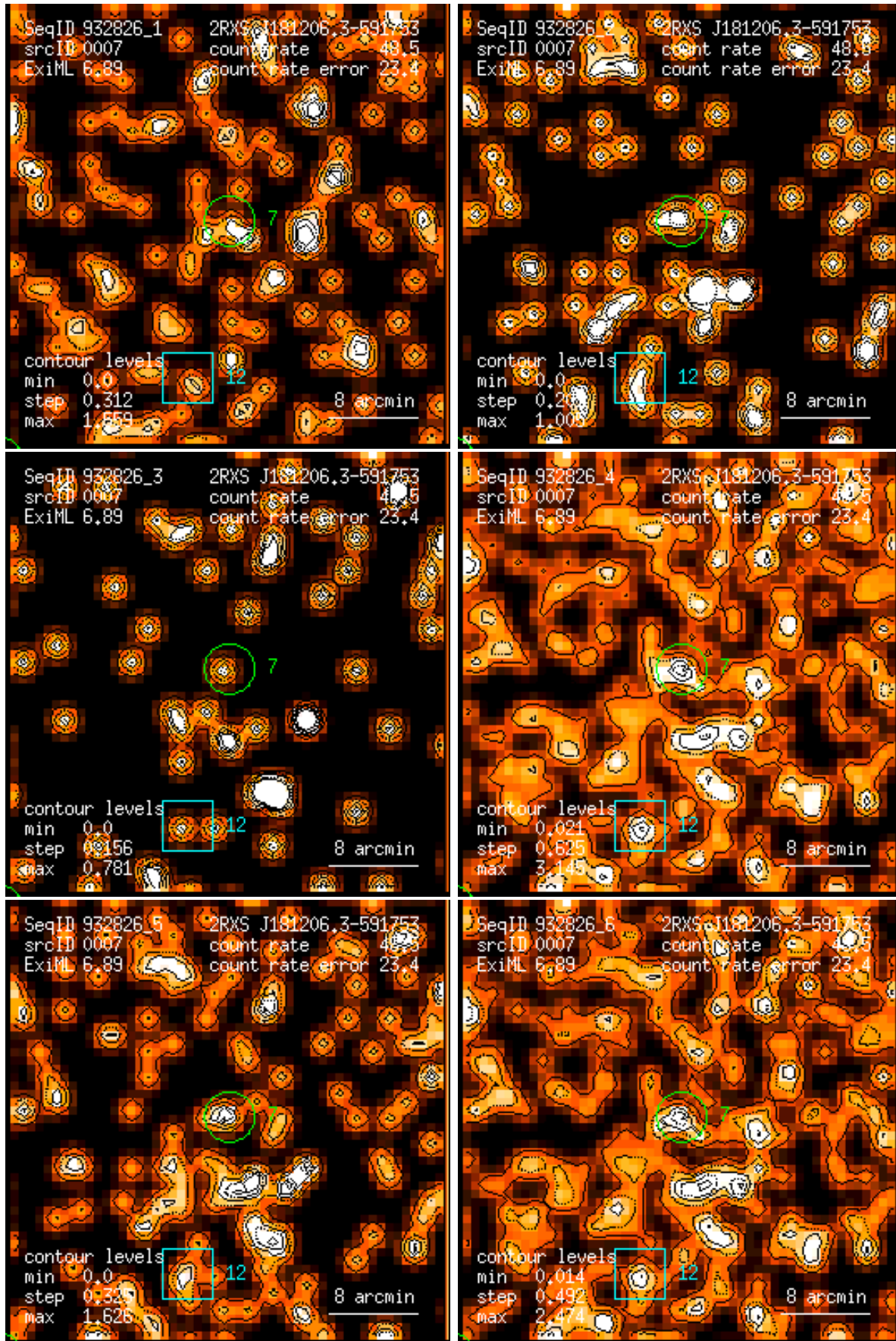
Figure 7: RASS 932826: detection 0007: band rate images, Gaussian filter: (1) PSPC channels 11 – 41, (2) 52 – 90, (3) 91 – 201, (4) 11 – 235, (5) 52 – 201, (6) 11 – 201. Broad band rates in counts/ks. Band rate contour levels in counts/ks/arcmin 2 .
