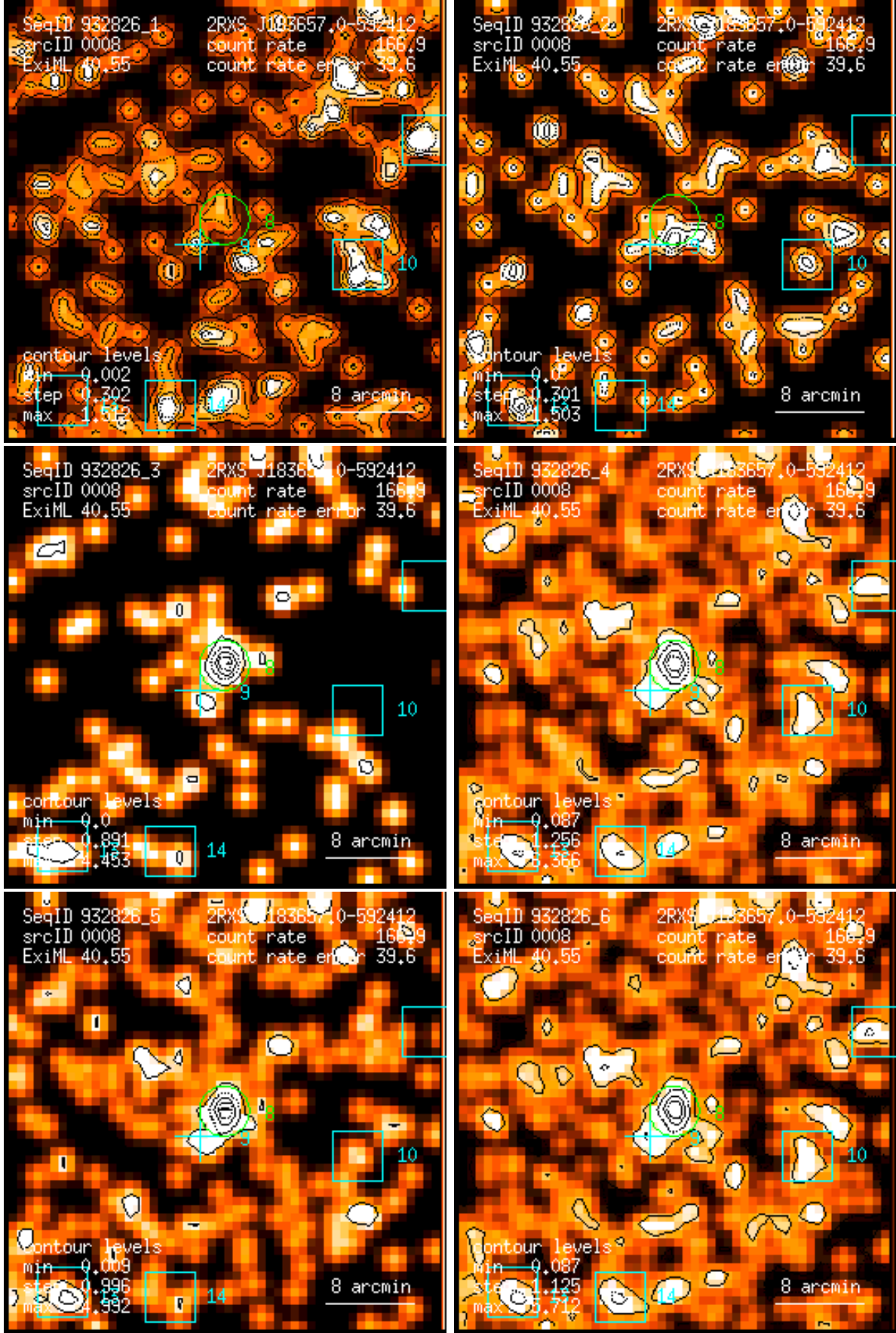
Figure 8: RASS 932826: detection 0008: band rate images, Gaussian filter: (1) PSPC channels 11 – 41, (2) 52 – 90, (3) 91 – 201, (4) 11 – 235, (5) 52 – 201, (6) 11 – 201. Broad band rates in counts/ks. Band rate contour levels in counts/ks/arcmin 2 .
