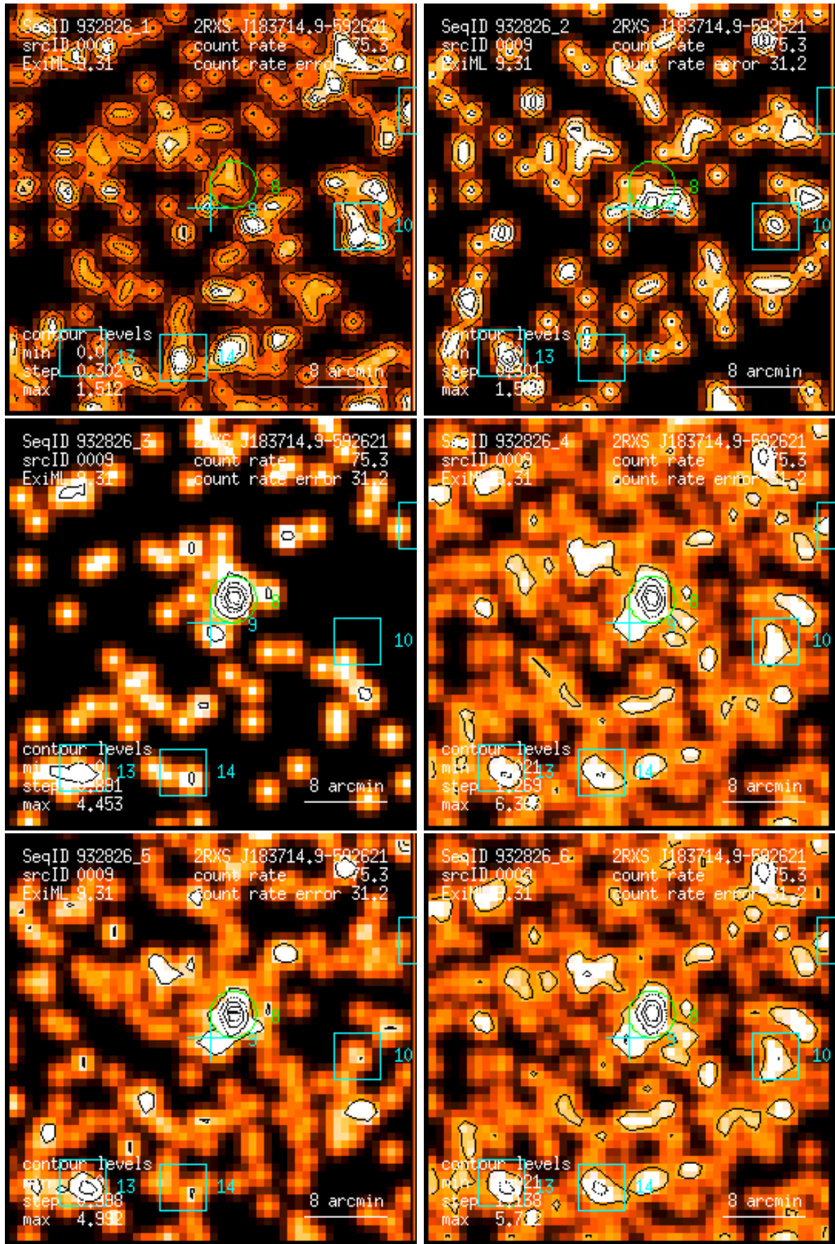
Figure 9: RASS 932826: detection 0009: band rate images, Gaussian filter: (1) PSPC channels 11 – 41, (2) 52 – 90, (3) 91 – 201, (4) 11 – 235, (5) 52 – 201, (6) 11 – 201. Broad band rates in counts/ks. Band rate contour levels in counts/ks/arcmin 2 .
