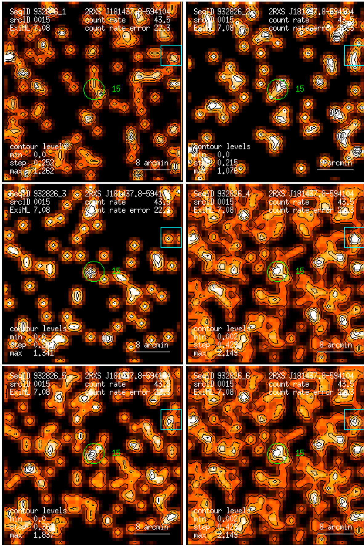
Figure 15: RASS 932826: detection 0015: band rate images, Gaussian filter: (1) PSPC channels 11 – 41, (2) 52 – 90, (3) 91 – 201, (4) 11 – 235, (5) 52 – 201, (6) 11 – 201. Broad band rates in counts/ks. Band rate contour levels in counts/ks/arcmin 2 .
