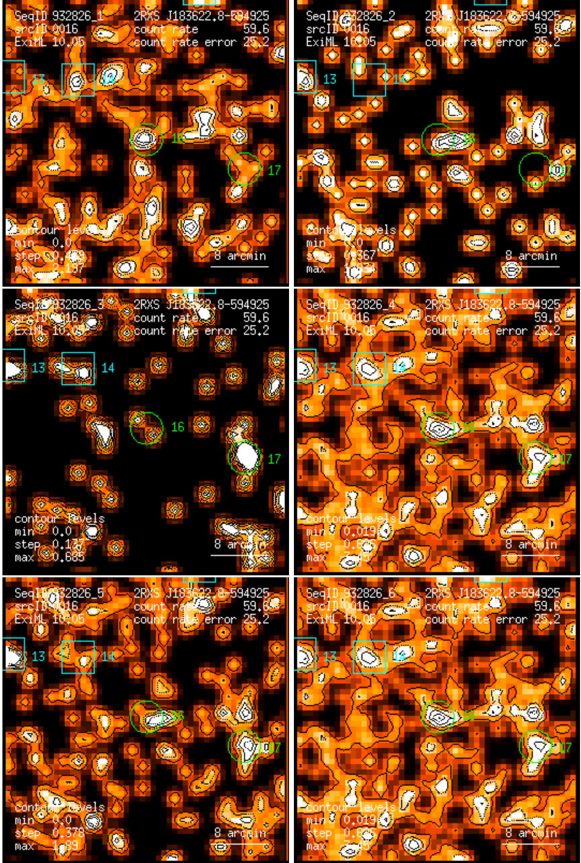
Figure 16: RASS 932826: detection 0016: band rate images, Gaussian filter: (1) PSPC channels 11 – 41, (2) 52 – 90, (3) 91 – 201, (4) 11 – 235, (5) 52 – 201, (6) 11 – 201. Broad band rates in counts/ks. Band rate contour levels in counts/ks/arcmin 2 .
