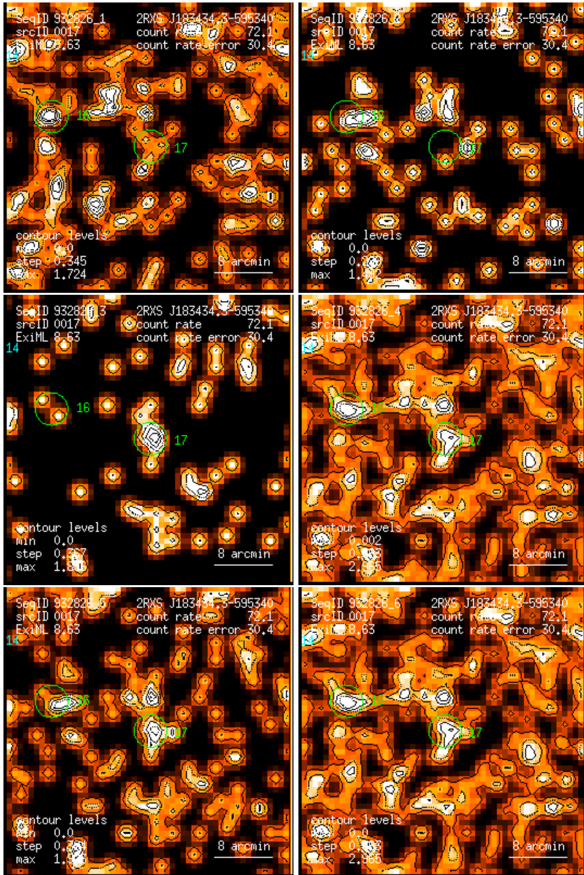
Figure 17: RASS 932826: detection 0017: band rate images, Gaussian filter: (1) PSPC channels 11 – 41, (2) 52 – 90, (3) 91 – 201, (4) 11 – 235, (5) 52 – 201, (6) 11 – 201. Broad band rates in counts/ks. Band rate contour levels in counts/ks/arcmin 2 .
