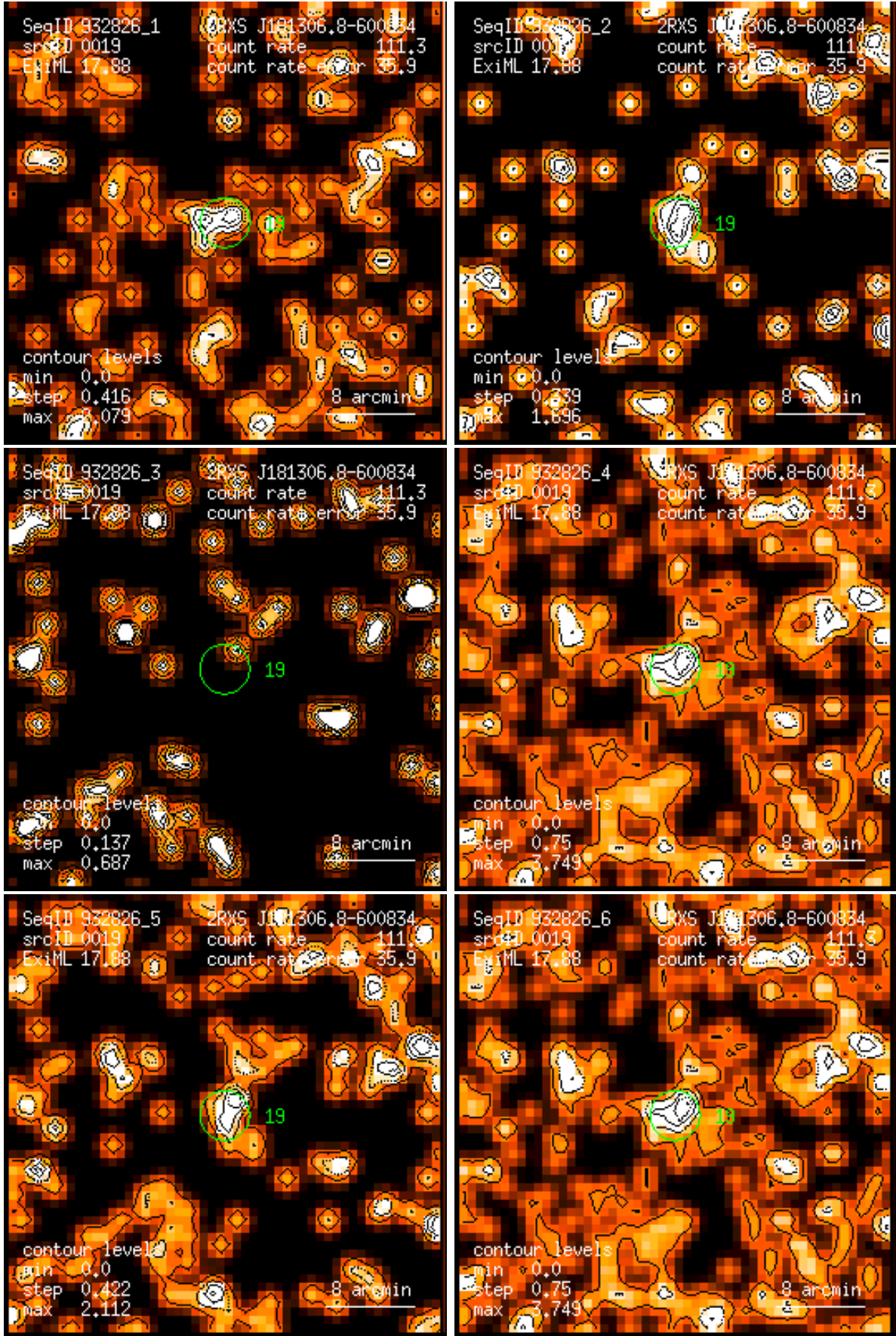
Figure 19: RASS 932826: detection 0019: band rate images, Gaussian filter: (1) PSPC channels 11 – 41, (2) 52 – 90, (3) 91 – 201, (4) 11 – 235, (5) 52 – 201, (6) 11 – 201. Broad band rates in counts/ks. Band rate contour levels in counts/ks/arcmin 2 .
