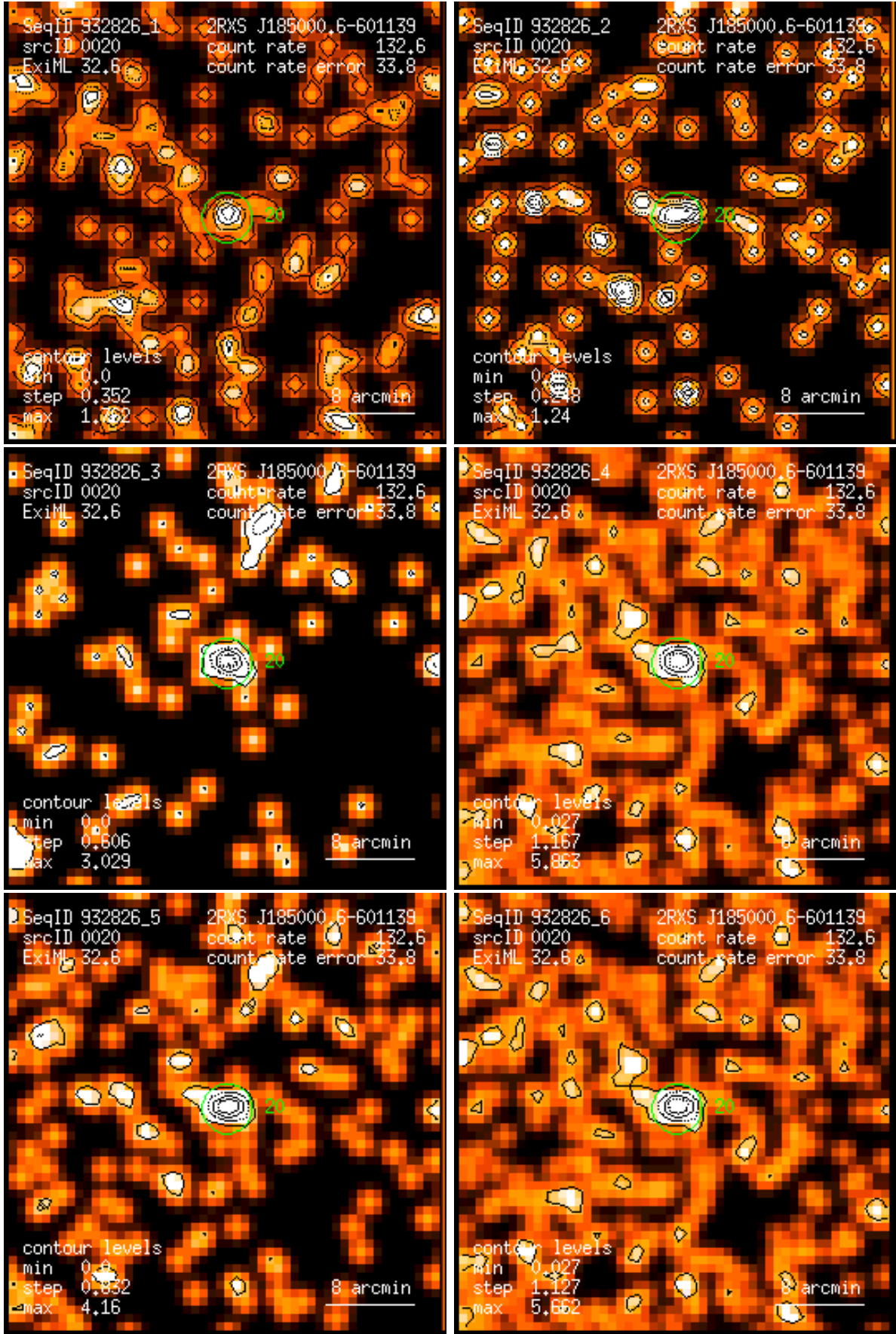
Figure 20: RASS 932826: detection 0020: band rate images, Gaussian filter: (1) PSPC channels 11 – 41, (2) 52 – 90, (3) 91 – 201, (4) 11 – 235, (5) 52 – 201, (6) 11 – 201. Broad band rates in counts/ks. Band rate contour levels in counts/ks/arcmin 2 .
