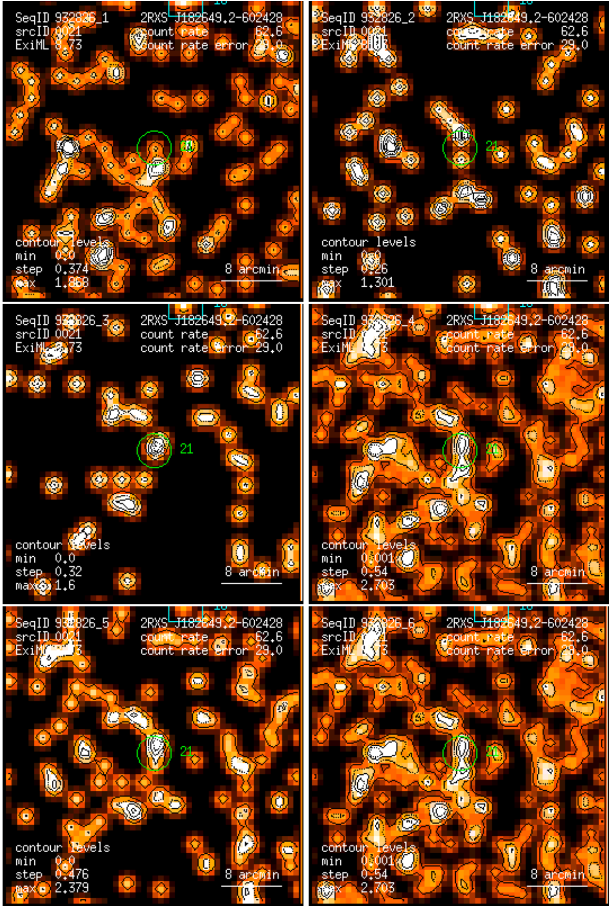
Figure 21: RASS 932826: detection 0021: band rate images, Gaussian filter: (1) PSPC channels 11 – 41, (2) 52 – 90, (3) 91 – 201, (4) 11 – 235, (5) 52 – 201, (6) 11 – 201. Broad band rates in counts/ks. Band rate contour levels in counts/ks/arcmin 2 .
