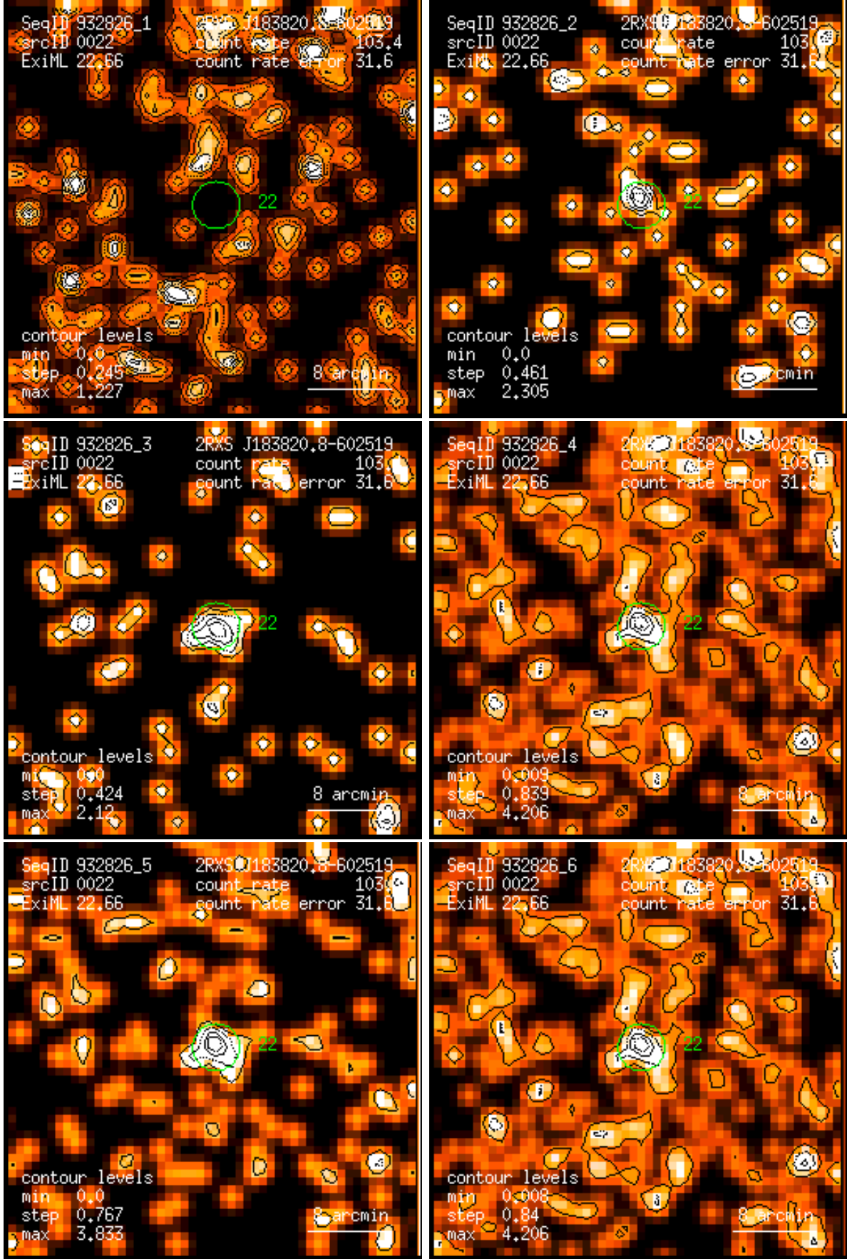
Figure 22: RASS 932826: detection 0022: band rate images, Gaussian filter: (1) PSPC channels 11 – 41, (2) 52 – 90, (3) 91 – 201, (4) 11 – 235, (5) 52 – 201, (6) 11 – 201. Broad band rates in counts/ks. Band rate contour levels in counts/ks/arcmin 2 .
