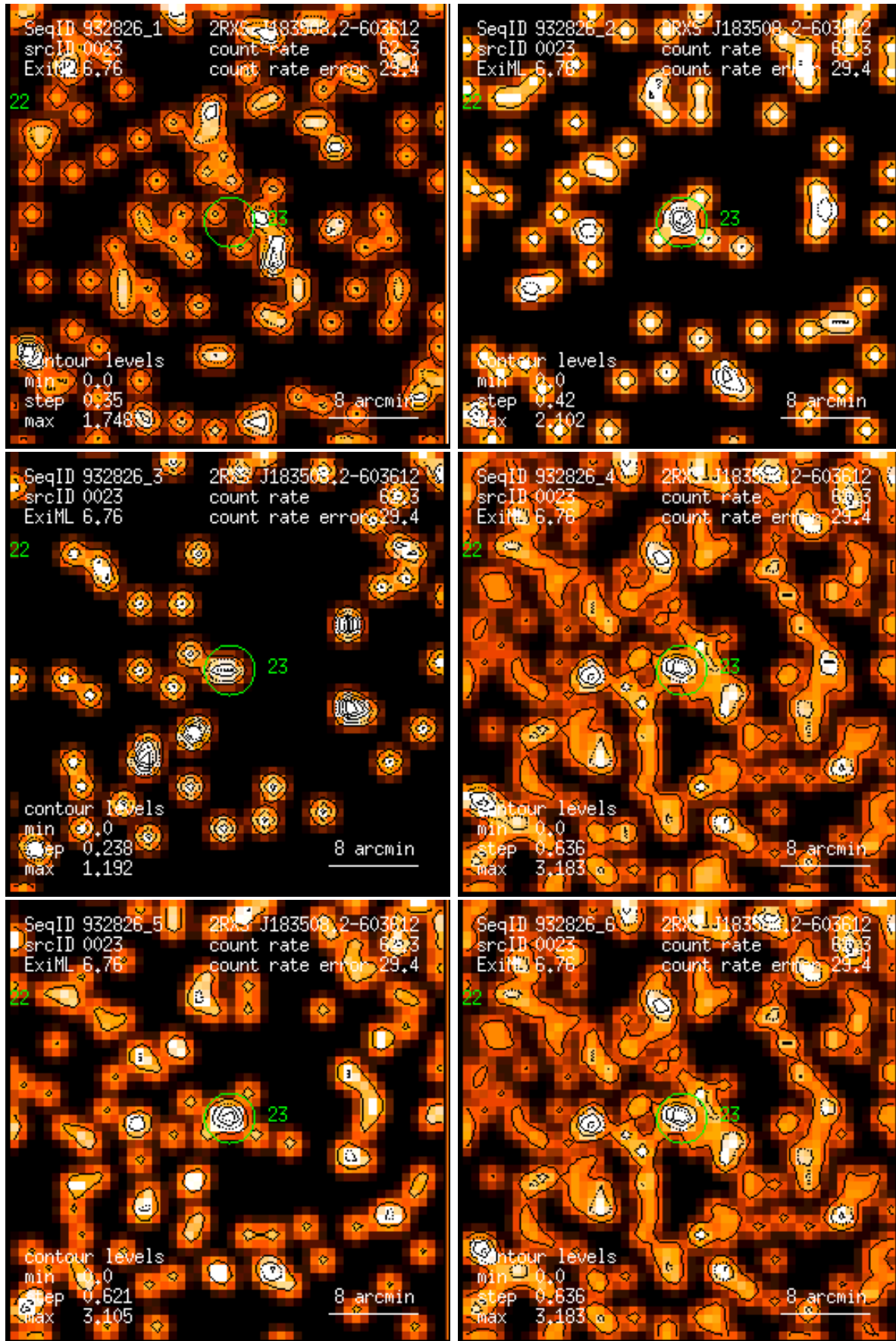
Figure 23: RASS 932826: detection 0023: band rate images, Gaussian filter: (1) PSPC channels 11 – 41, (2) 52 – 90, (3) 91 – 201, (4) 11 – 235, (5) 52 – 201, (6) 11 – 201. Broad band rates in counts/ks. Band rate contour levels in counts/ks/arcmin 2 .
