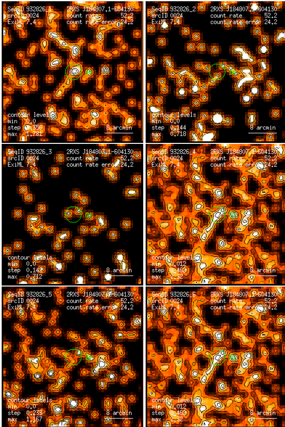
Figure 24: RASS 932826: detection 0024: band rate images, Gaussian filter: (1) PSPC channels 11 – 41, (2) 52 – 90, (3) 91 – 201, (4) 11 – 235, (5) 52 – 201, (6) 11 – 201. Broad band rates in counts/ks. Band rate contour levels in counts/ks/arcmin 2 .
