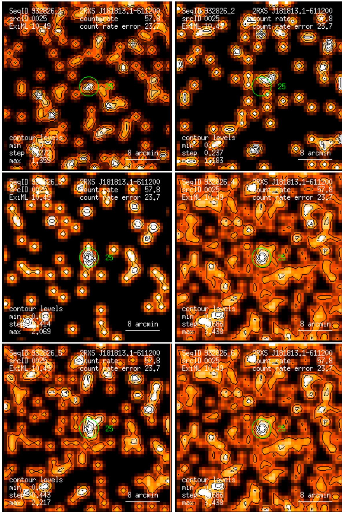
Figure 25: RASS 932826: detection 0025: band rate images, Gaussian filter: (1) PSPC channels 11 – 41, (2) 52 – 90, (3) 91 – 201, (4) 11 – 235, (5) 52 – 201, (6) 11 – 201. Broad band rates in counts/ks. Band rate contour levels in counts/ks/arcmin 2 .
