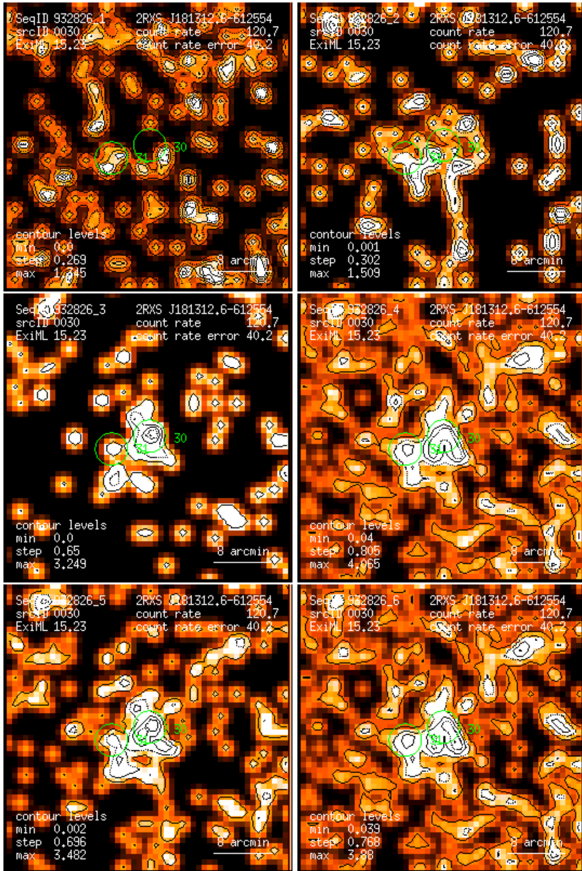
Figure 30: RASS 932826: detection 0030: band rate images, Gaussian filter: (1) PSPC channels 11 – 41, (2) 52 – 90, (3) 91 – 201, (4) 11 – 235, (5) 52 – 201, (6) 11 – 201. Broad band rates in counts/ks. Band rate contour levels in counts/ks/arcmin 2 .
