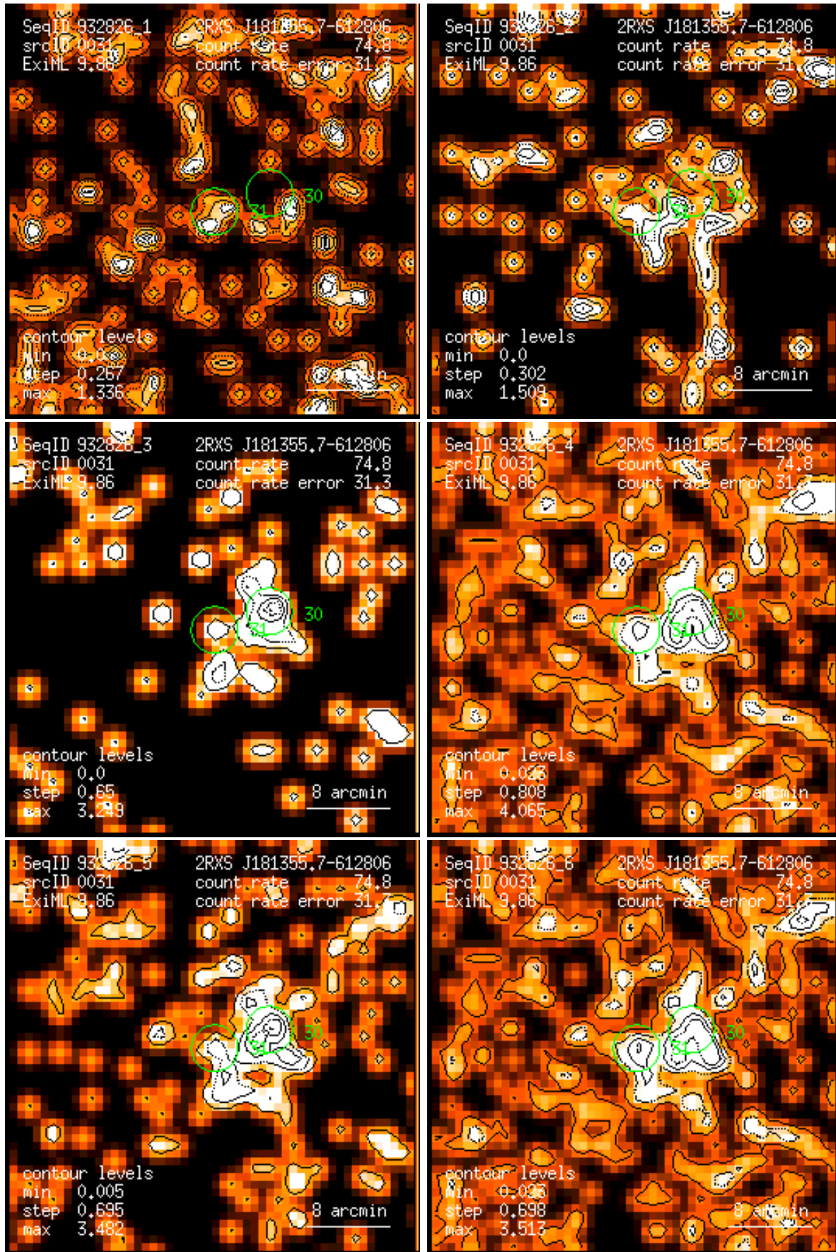
Figure 31: RASS 932826: detection 0031: band rate images, Gaussian filter: (1) PSPC channels 11 – 41, (2) 52 – 90, (3) 91 – 201, (4) 11 – 235, (5) 52 – 201, (6) 11 – 201. Broad band rates in counts/ks. Band rate contour levels in counts/ks/arcmin 2 .
