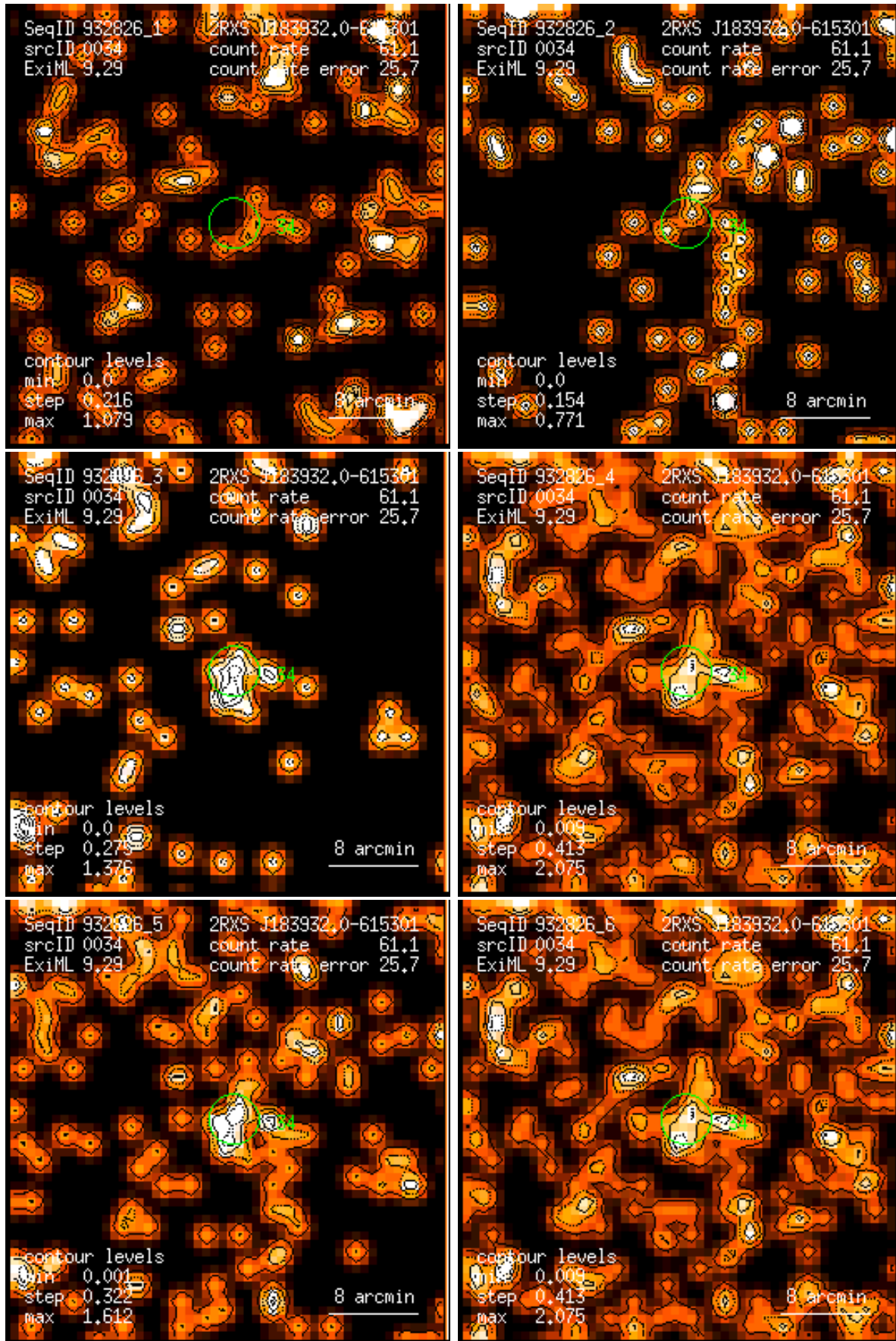
Figure 34: RASS 932826: detection 0034: band rate images, Gaussian filter: (1) PSPC channels 11 – 41, (2) 52 – 90, (3) 91 – 201, (4) 11 – 235, (5) 52 – 201, (6) 11 – 201. Broad band rates in counts/ks. Band rate contour levels in counts/ks/arcmin 2 .
