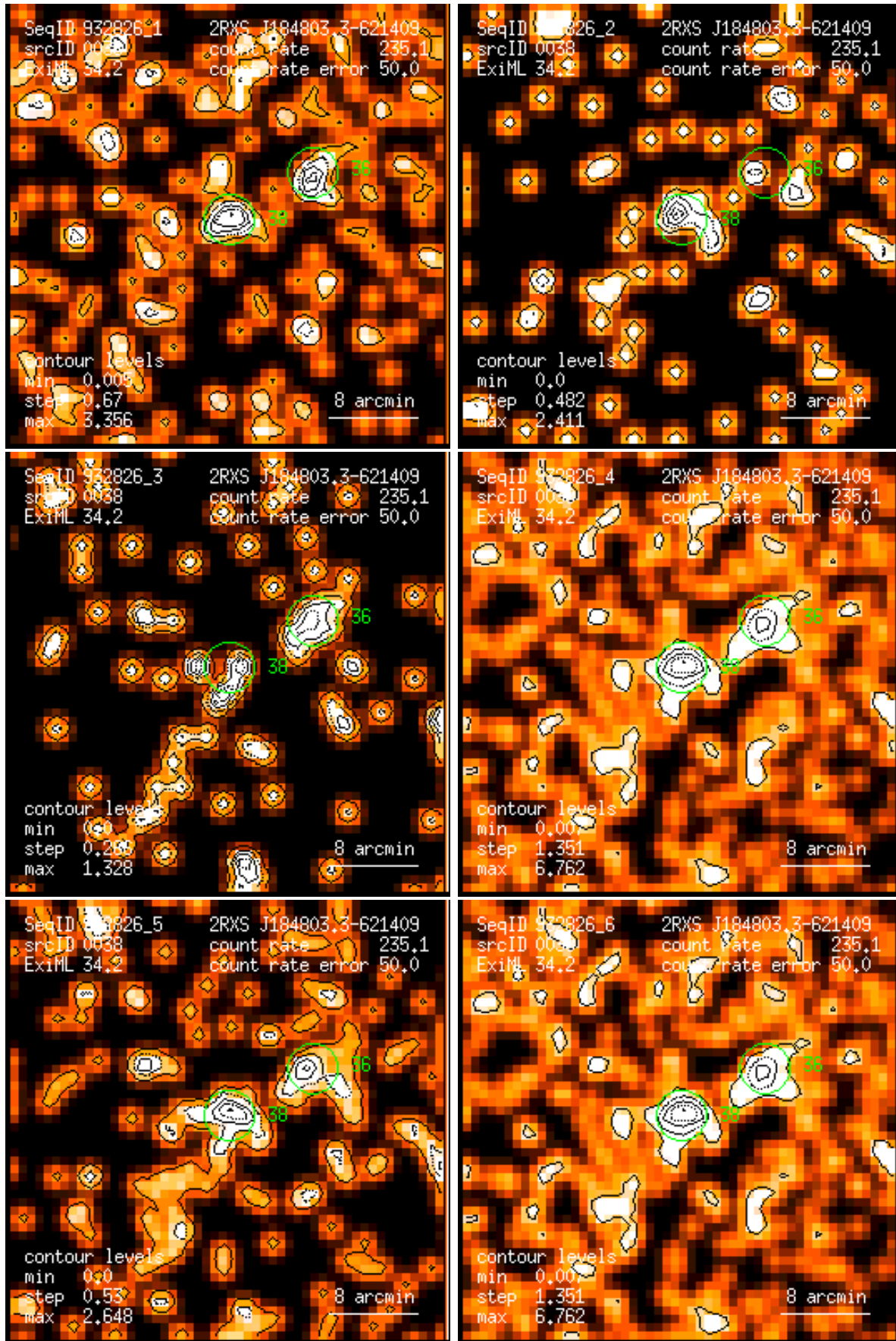
Figure 38: RASS 932826: detection 0038: band rate images, Gaussian filter: (1) PSPC channels 11 – 41, (2) 52 – 90, (3) 91 – 201, (4) 11 – 235, (5) 52 – 201, (6) 11 – 201. Broad band rates in counts/ks. Band rate contour levels in counts/ks/arcmin 2 .
