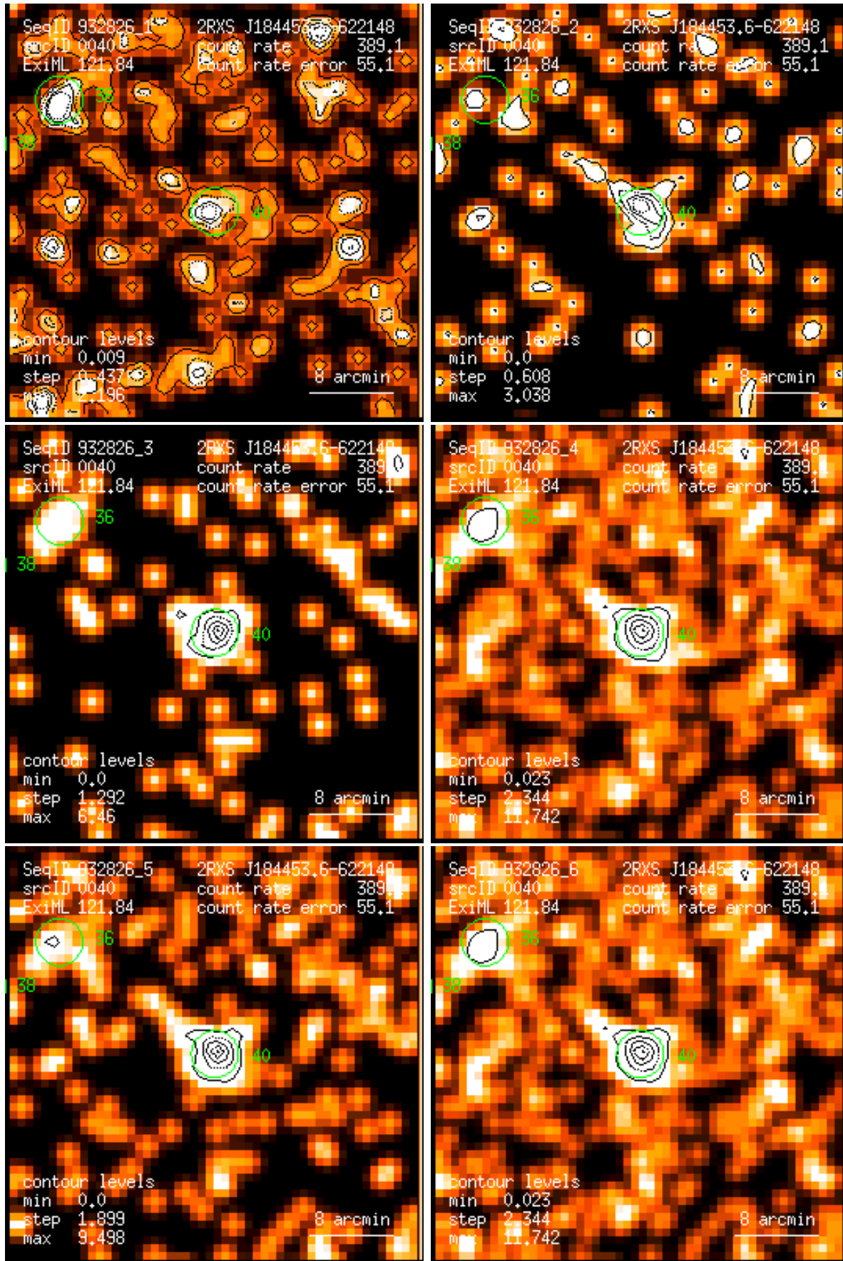
Figure 40: RASS 932826: detection 0040: band rate images, Gaussian filter: (1) PSPC channels 11 – 41, (2) 52 – 90, (3) 91 – 201, (4) 11 – 235, (5) 52 – 201, (6) 11 – 201. Broad band rates in counts/ks. Band rate contour levels in counts/ks/arcmin 2 .
