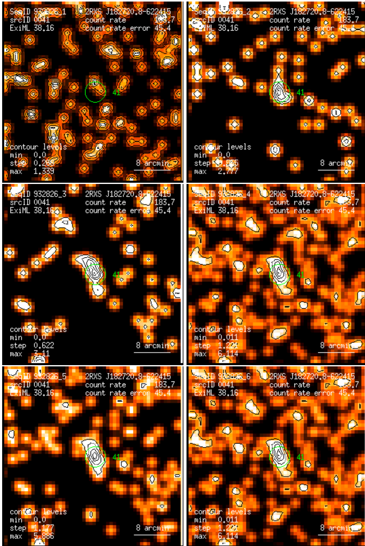
Figure 41: RASS 932826: detection 0041: band rate images, Gaussian filter: (1) PSPC channels 11 – 41, (2) 52 – 90, (3) 91 – 201, (4) 11 – 235, (5) 52 – 201, (6) 11 – 201. Broad band rates in counts/ks. Band rate contour levels in counts/ks/arcmin 2 .
