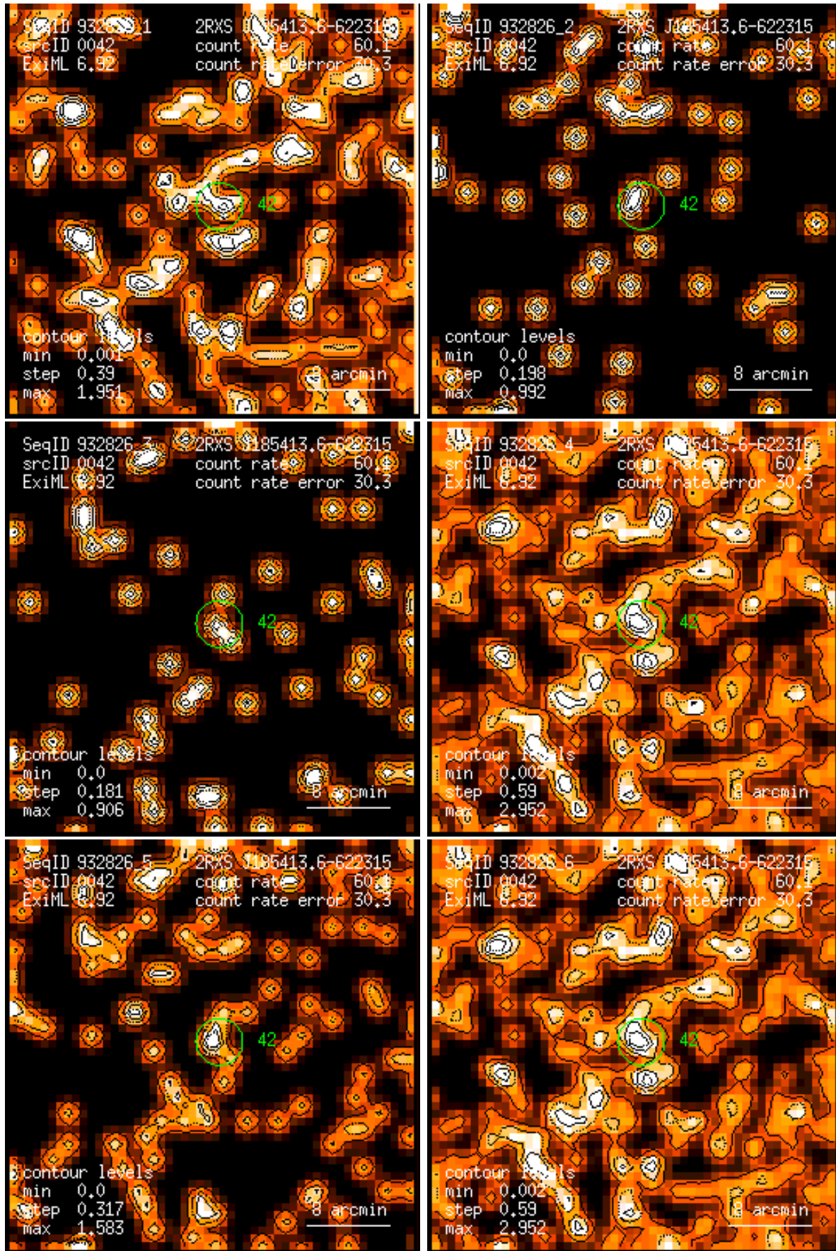
Figure 42: RASS 932826: detection 0042: band rate images, Gaussian filter: (1) PSPC channels 11 – 41, (2) 52 – 90, (3) 91 – 201, (4) 11 – 235, (5) 52 – 201, (6) 11 – 201. Broad band rates in counts/ks. Band rate contour levels in counts/ks/arcmin 2 .
