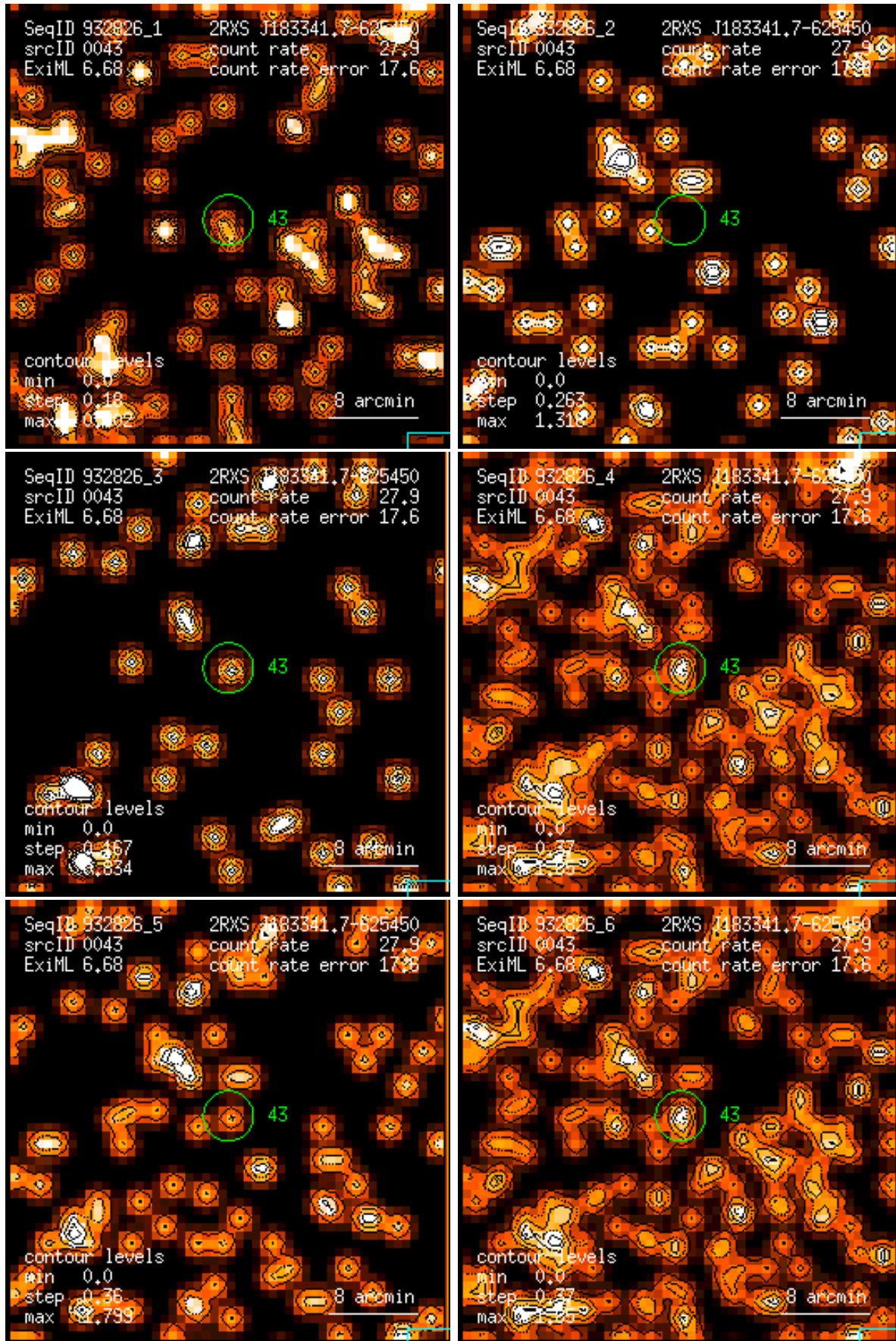
Figure 43: RASS 932826: detection 0043: band rate images, Gaussian filter: (1) PSPC channels 11 – 41, (2) 52 – 90, (3) 91 – 201, (4) 11 – 235, (5) 52 – 201, (6) 11 – 201. Broad band rates in counts/ks. Band rate contour levels in counts/ks/arcmin 2 .
