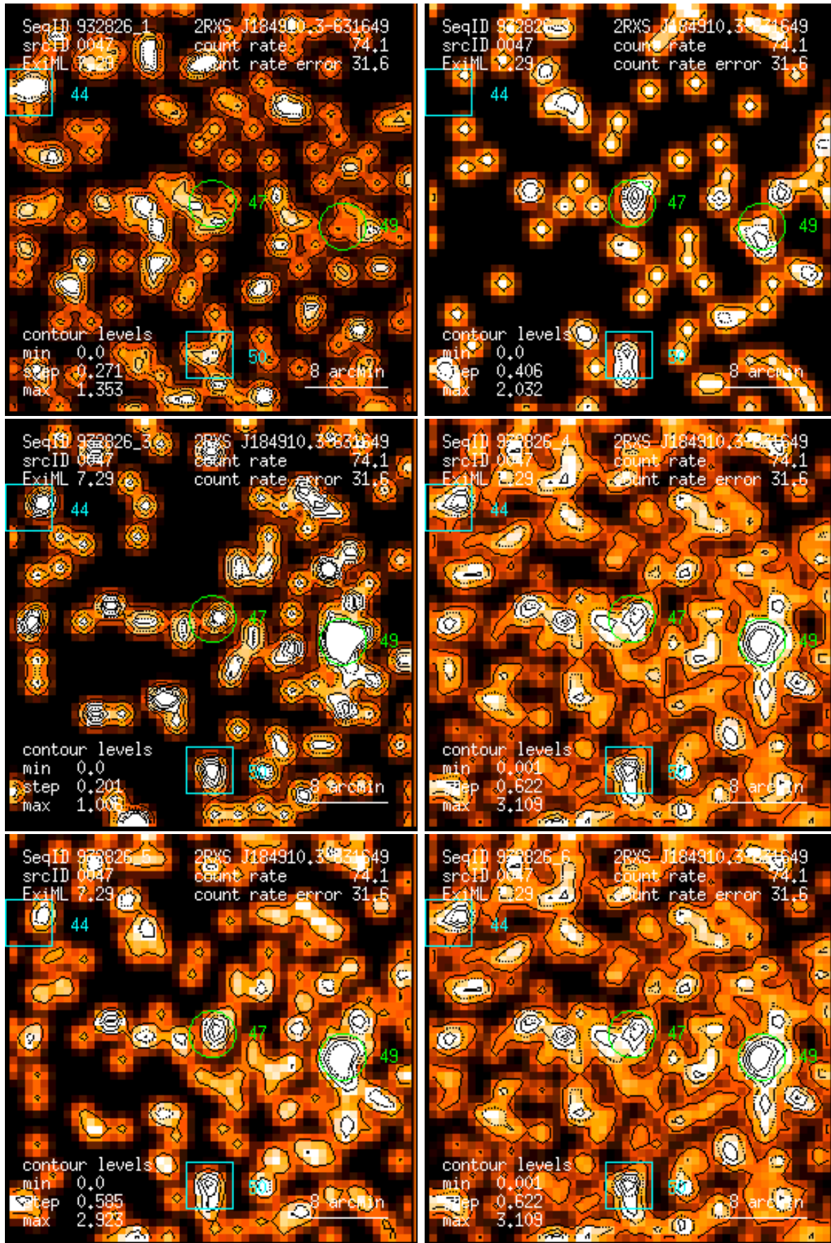
Figure 47: RASS 932826: detection 0047: band rate images, Gaussian filter: (1) PSPC channels 11 – 41, (2) 52 – 90, (3) 91 – 201, (4) 11 – 235, (5) 52 – 201, (6) 11 – 201. Broad band rates in counts/ks. Band rate contour levels in counts/ks/arcmin 2 .
