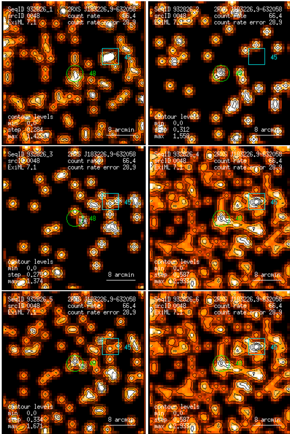
Figure 48: RASS 932826: detection 0048: band rate images, Gaussian filter: (1) PSPC channels 11 – 41, (2) 52 – 90, (3) 91 – 201, (4) 11 – 235, (5) 52 – 201, (6) 11 – 201. Broad band rates in counts/ks. Band rate contour levels in counts/ks/arcmin 2 .
