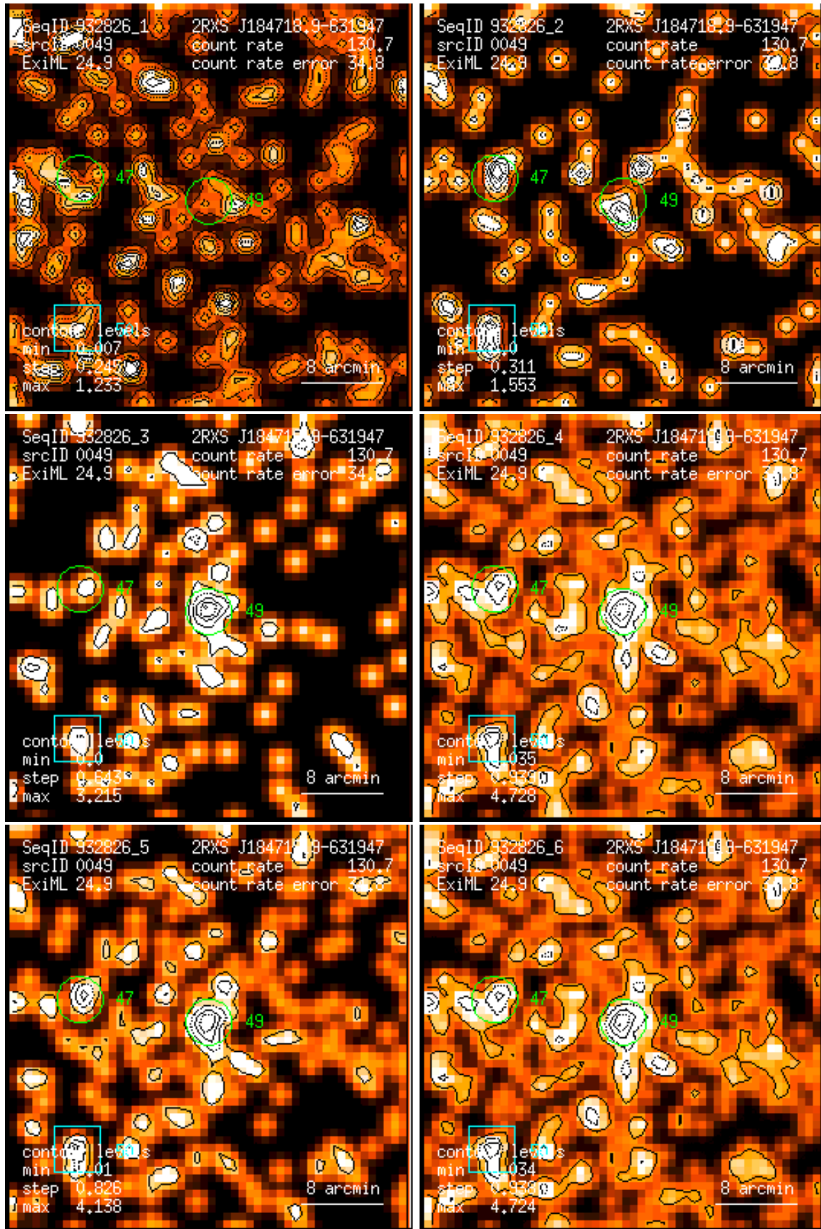
Figure 49: RASS 932826: detection 0049: band rate images, Gaussian filter: (1) PSPC channels 11 – 41, (2) 52 – 90, (3) 91 – 201, (4) 11 – 235, (5) 52 – 201, (6) 11 – 201. Broad band rates in counts/ks. Band rate contour levels in counts/ks/arcmin 2 .
