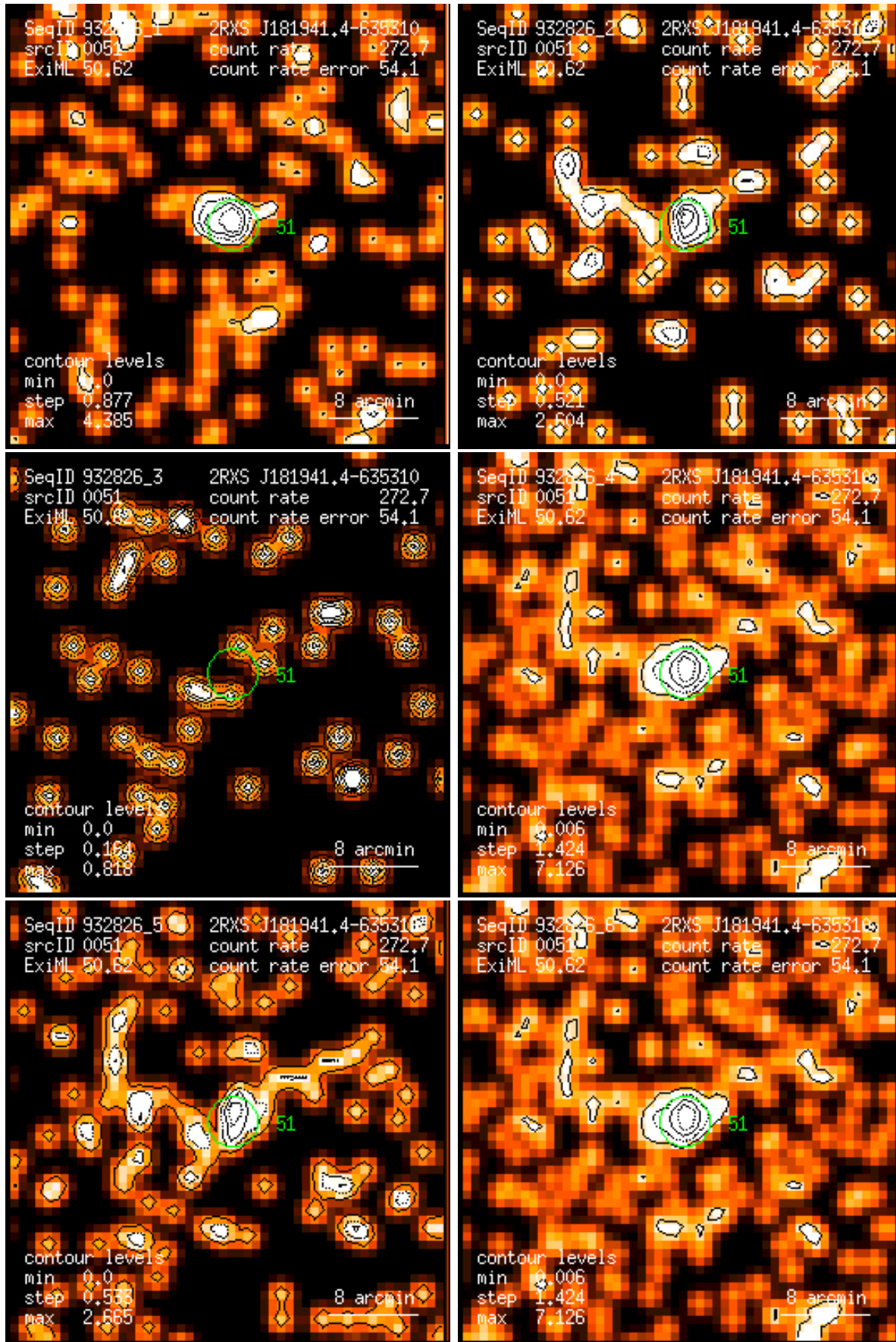
Figure 51: RASS 932826: detection 0051: band rate images, Gaussian filter: (1) PSPC channels 11 – 41, (2) 52 – 90, (3) 91 – 201, (4) 11 – 235, (5) 52 – 201, (6) 11 – 201. Broad band rates in counts/ks. Band rate contour levels in counts/ks/arcmin 2 .
