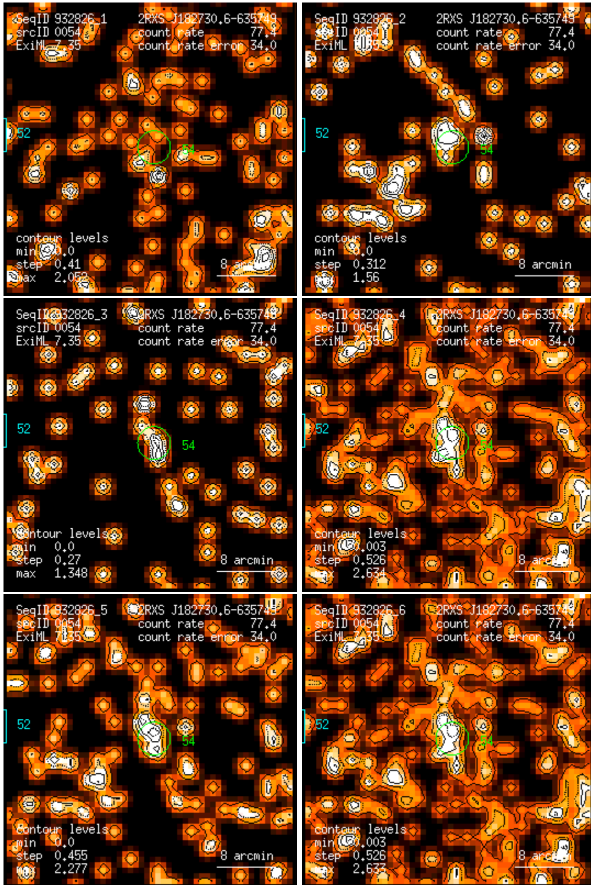
Figure 54: RASS 932826: detection 0054: band rate images, Gaussian filter: (1) PSPC channels 11 – 41, (2) 52 – 90, (3) 91 – 201, (4) 11 – 235, (5) 52 – 201, (6) 11 – 201. Broad band rates in counts/ks. Band rate contour levels in counts/ks/arcmin 2 .
